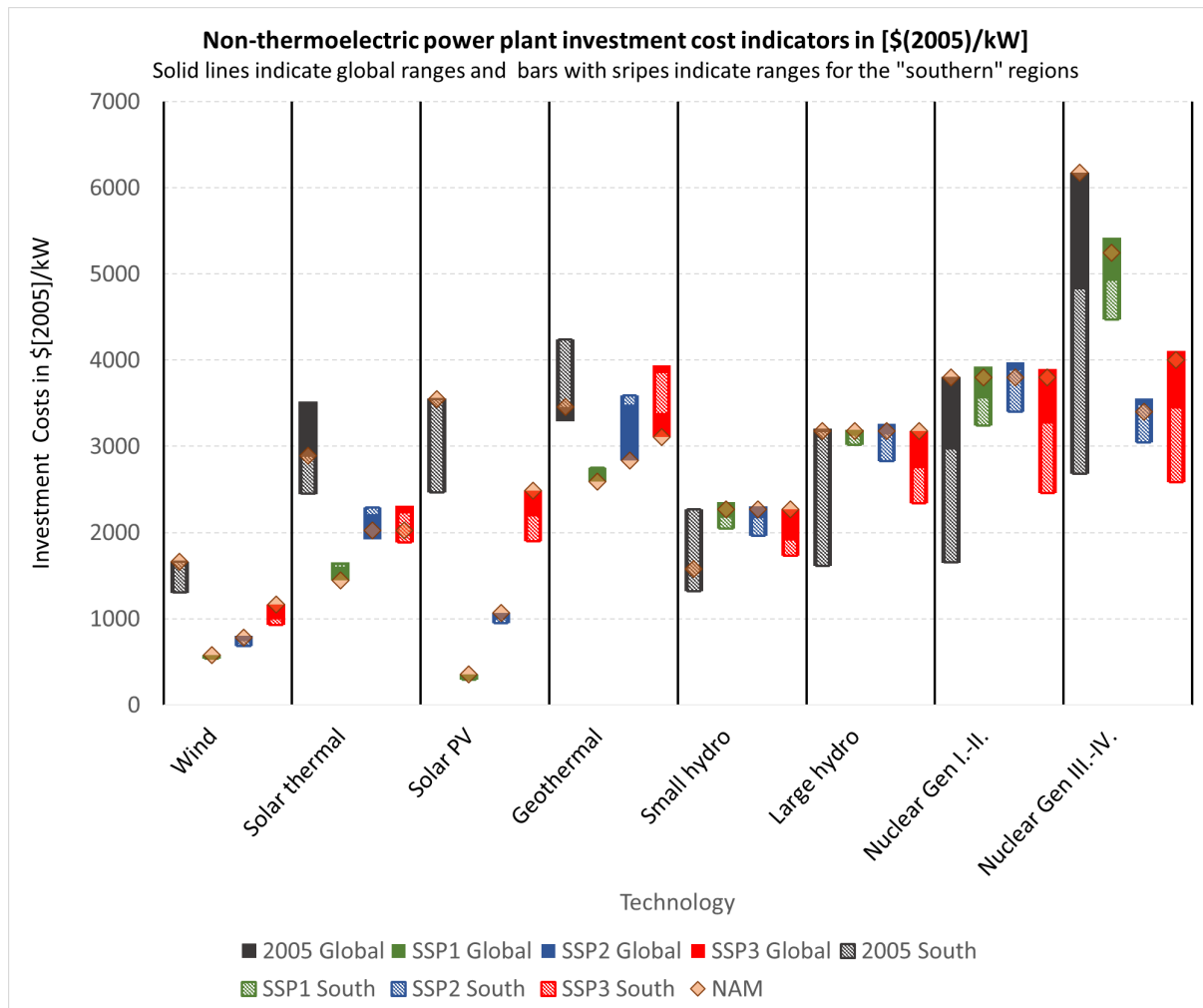
Fig. 3.7: Cost indicators for non-thermoelectric power-plant investment (Fricko et al., 2017 [[17]]). Abbreviations: CCS – Carbon Capture and Storage; IGCC – Integrated gasification combined cycles; ST – Steam turbine; CT – Combustion turbine; CCGT – Combined cycle gas turbine
