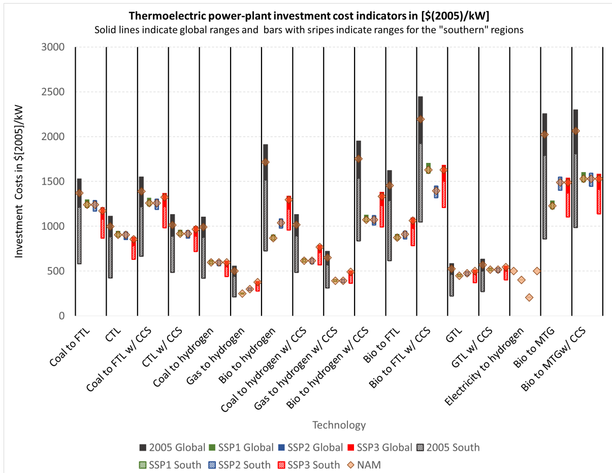
Fig. 3.8: Cost indicators for other conversion technology investment (Fricko et al., 2017 [[17]]) Abbreviations: CCS – Carbon capture and storage; CTL – Coal to liquids; GTL – Gas to liquids; BTL – Biomass to liquids.
