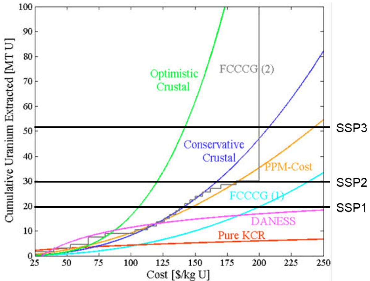
Fig. 3.2: Global uranium resources in the MESSAGE interpretation of the SSPs compared to seven supply curves from a literature review (Schneider and Sailor, 2008 [[96]]). Conservative Crustal and Optimistic Crustal refer to simple crustal models of uranium distribution in the crust and the of extraction costs on the concentration. Pure-KCR refers to a fit of a simple crustal model to known conventional resources (KCR) as estimated by the Red Book 2003 (OECD/NEA, 2004 [[112]]). PPM-Cost over the simple crustal models include a relationship between uranium grade and extraction costs. FCCCG(1) and (2) as well as DANESS refer to estimats from more complicated models of the dependency of extraction costs on uranium concentration (and therefore resource grade).
