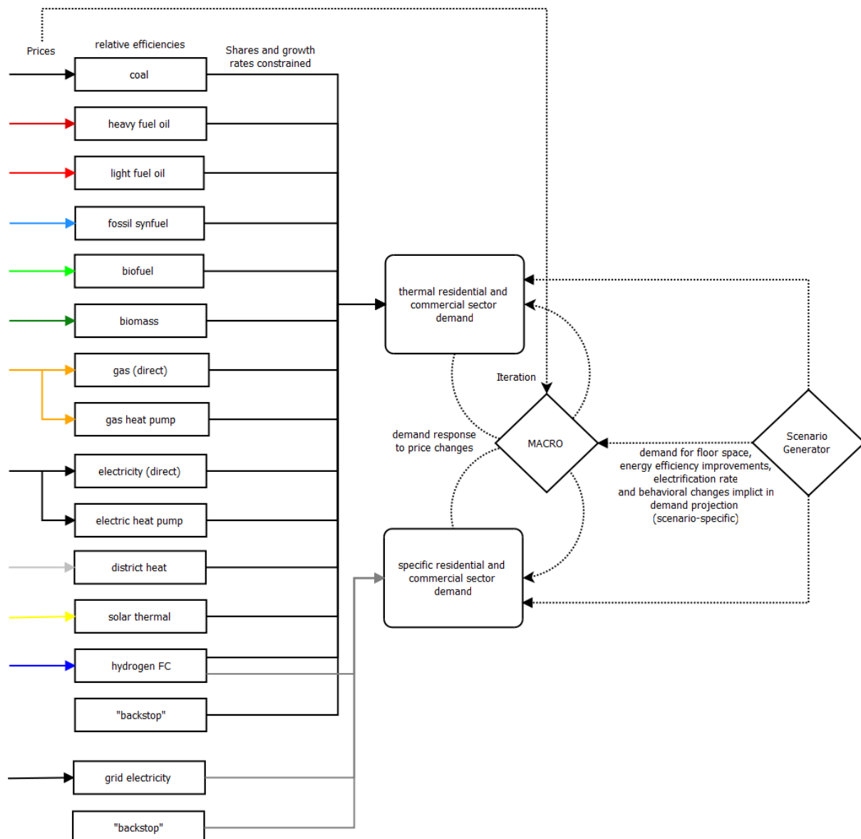
Fig. 3.11: Schematic diagram of the residential and commercial sector representation in MESSAGEix.
