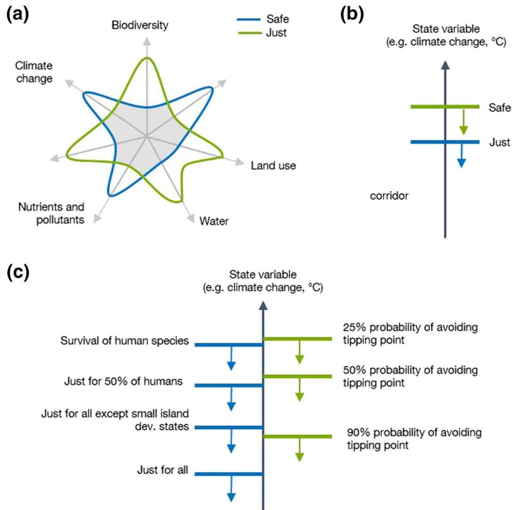
Figure 2. Integration of safe and just targets into the corridor. (a) For each biophysical variable, safe and just target ranges are identified. (b) We define the corridor (shaded) as the stricter of the safe and just ranges. In this example, the just range is stricter than the safe range. (c) We propose to identify a spread of safe and just target ranges corresponding to different risk tolerances. The variables and targets shown are strictly examples only.
