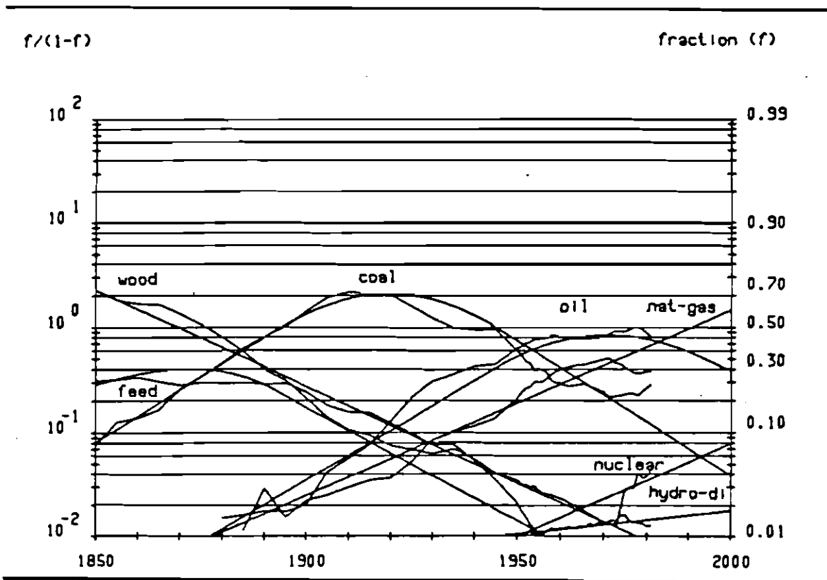
Figure 2.2 Primary Energy Substitution (since 1850).
