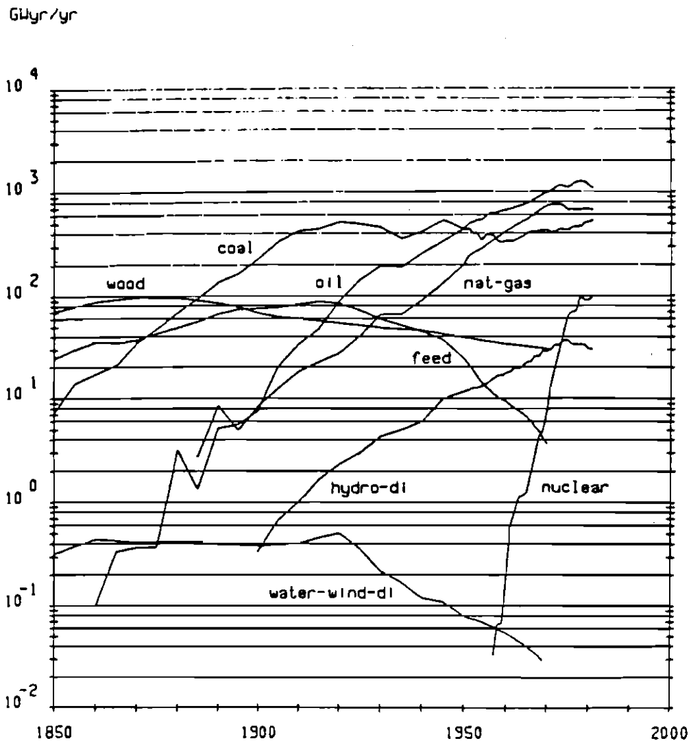
Figure 2.1 Primary Energy Consumption (since 1850).
