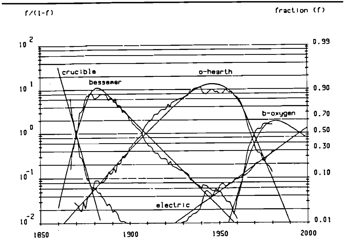
Figure 2.6 Technological Substitution in Steel Production.
