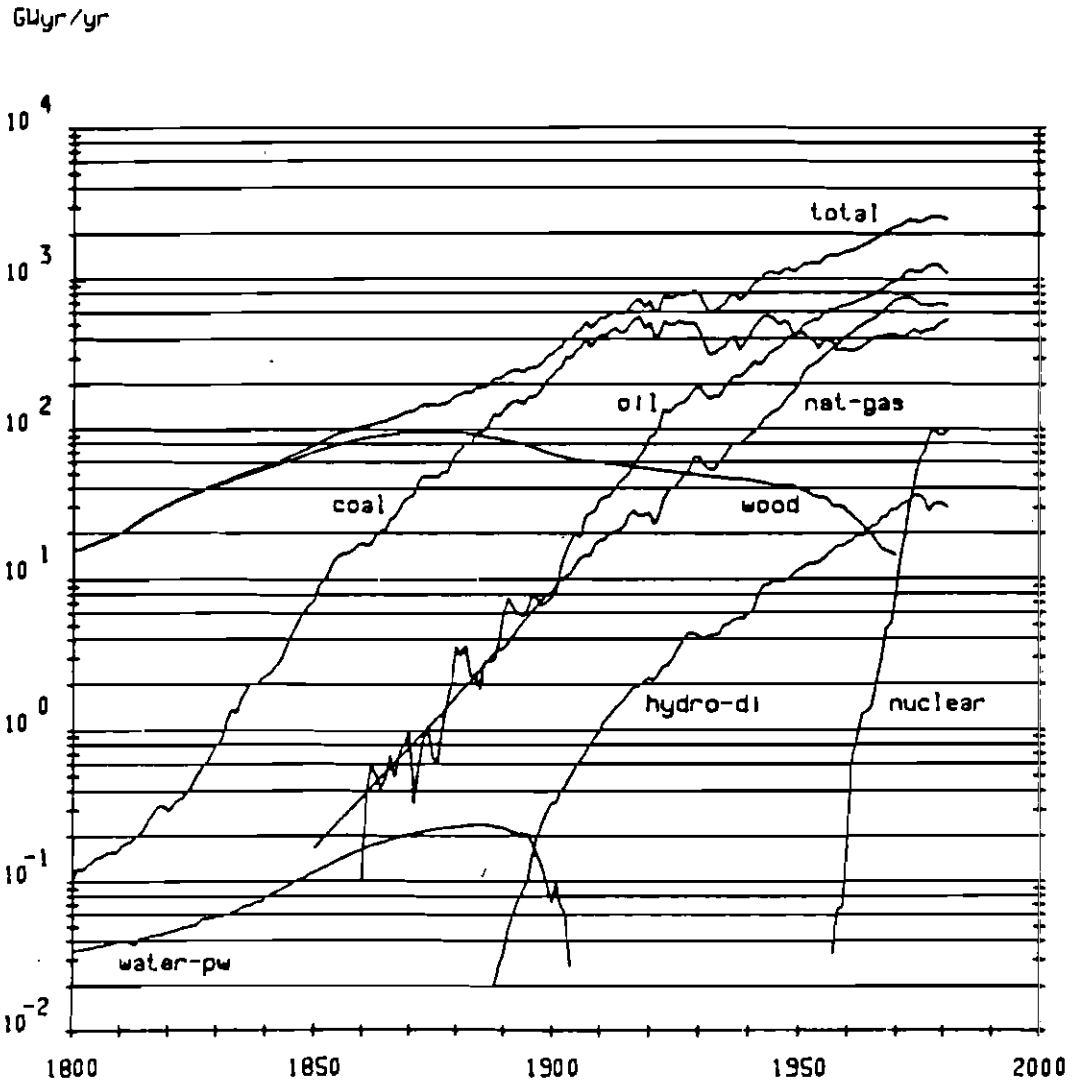
Figure 2.3 Primary Energy Consumption (since 1800).
