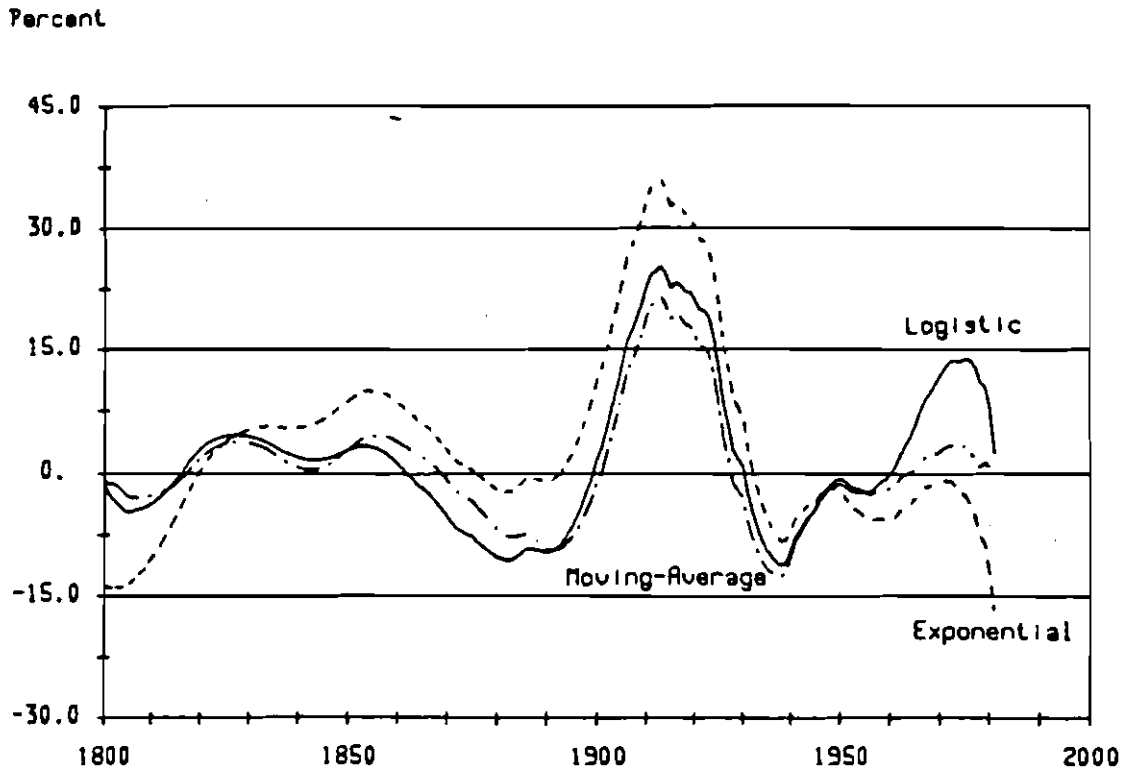
Figure 3.4 Long Wave in Primary Energy Consumption (three estimates).
