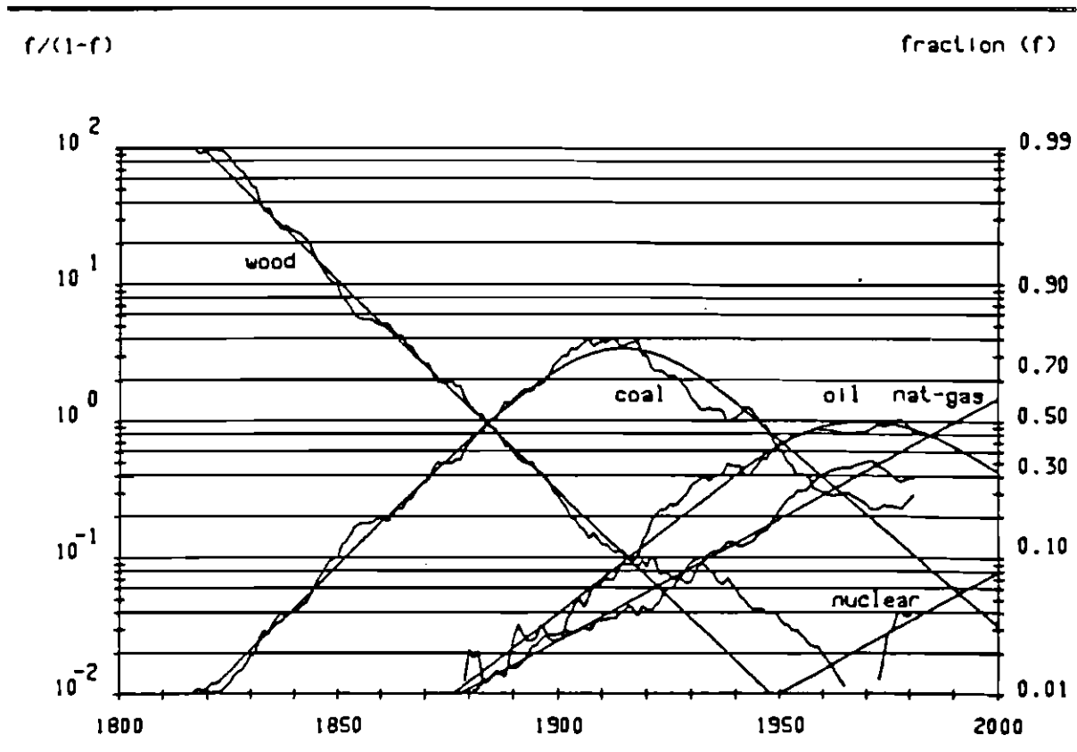
Figure 2.4 Primary Energy Substitution (since 1800).
