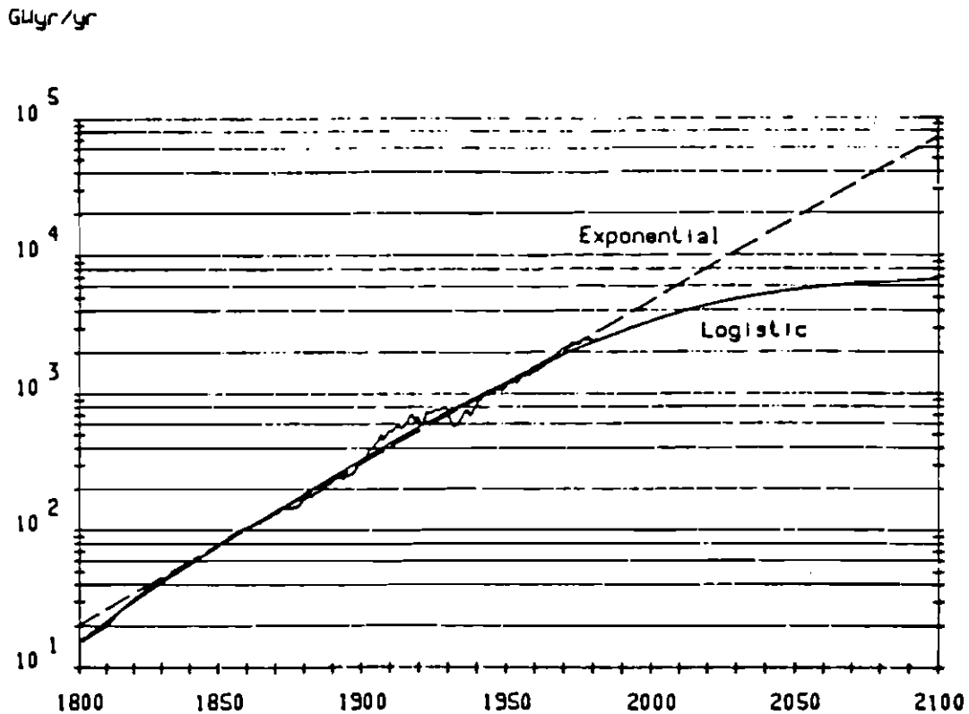
Figure 3.3 Primary Energy Consumption (with two secular trends).
