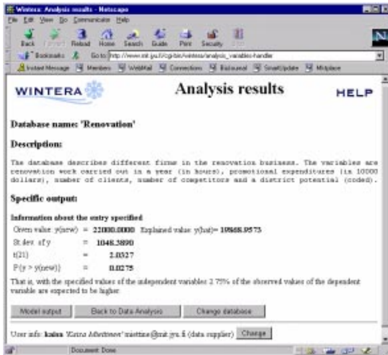
Figure 4. Specific output of WINTERA
