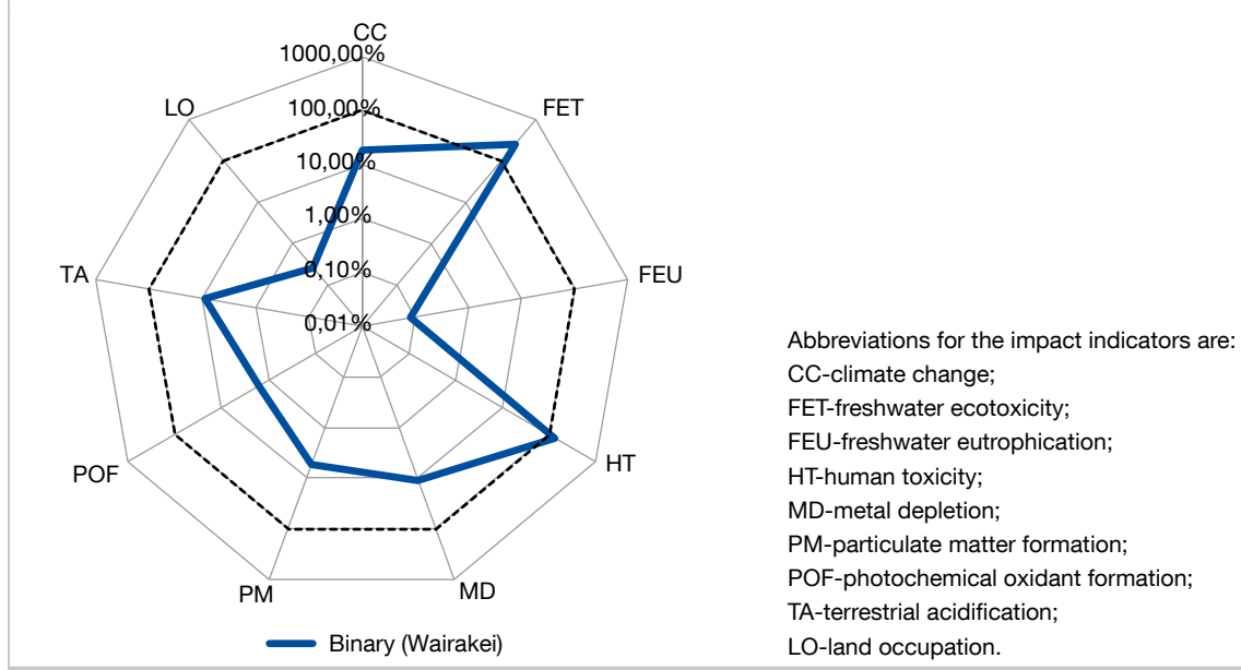
Environmental impacts for a 177 MW geothermal plant (Wairakei) relative to the OECD Pacific electricity mix of 2010
