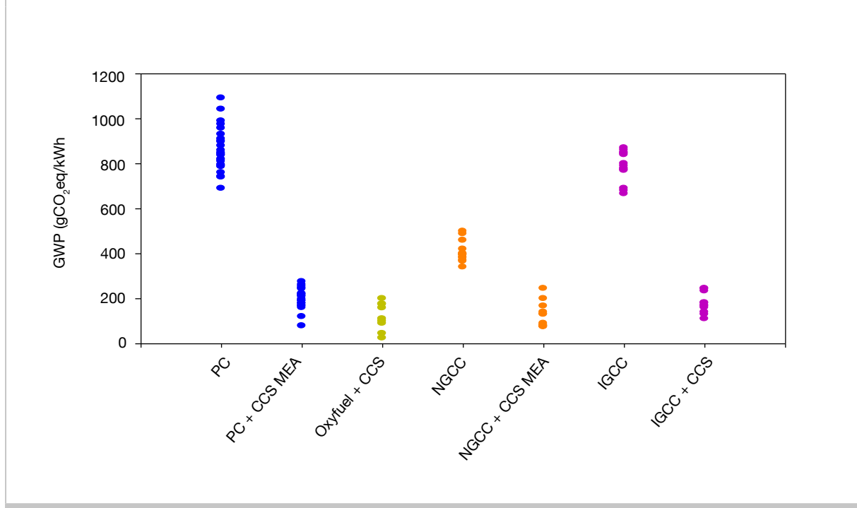
Global warming potential of power plants with and without CCS
