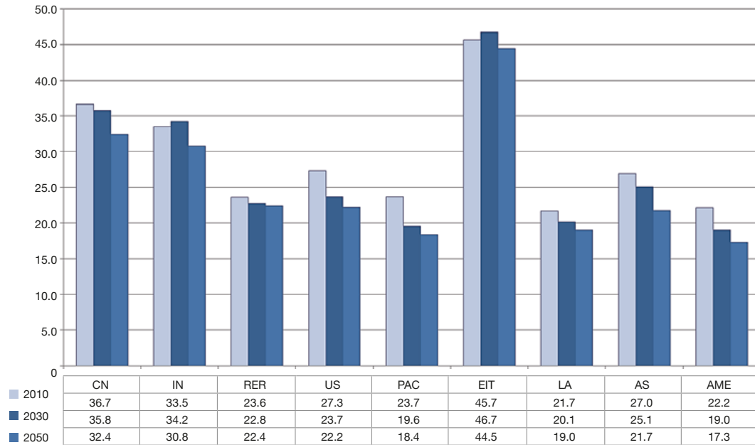
Regional comparison of impacts on climate change from a parabolic trough CSP plant
