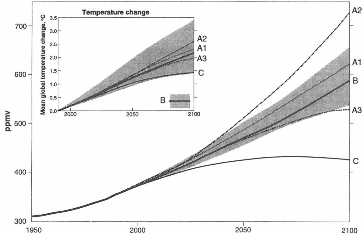
Fig. 10. CO 2 concentrations (ppmv), 1950 to 2100, and global mean temperature change (°C), 1990 to 2100. The (substantial) model uncertainties are indicated for Case B.
