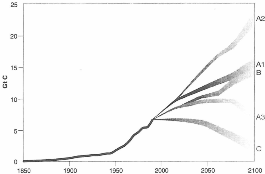
Fig. 9. Global energy-related carbon emissions, 1850 to 1990, and for three scenario families to 2100, in GtC.
