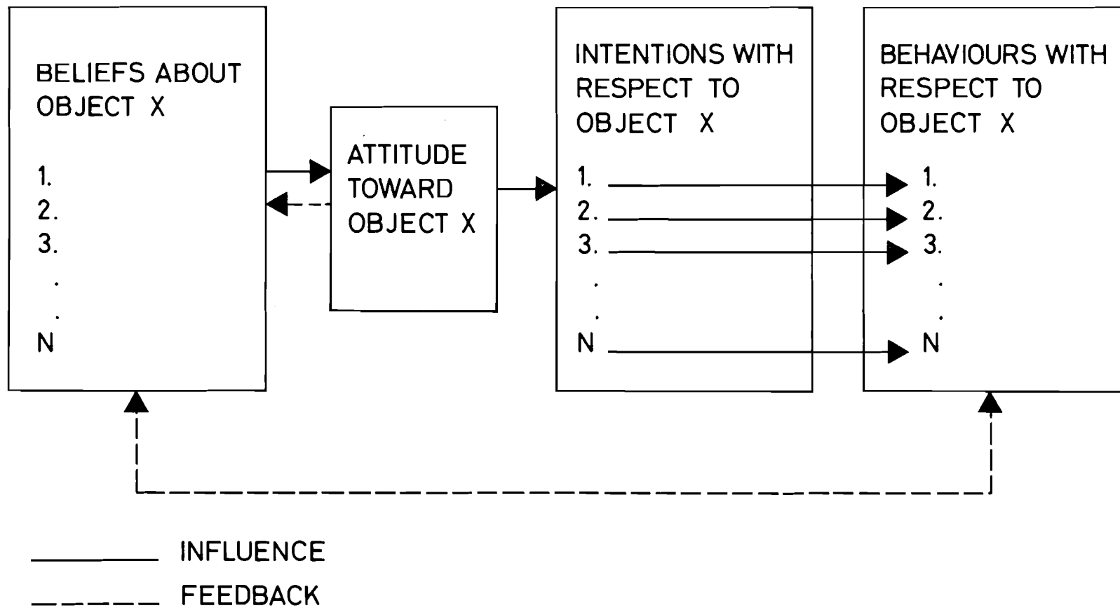
Schematic presentation of conceptual framework relating beliefs, attitudes, intentions, and behaviours with respect to a given object.
