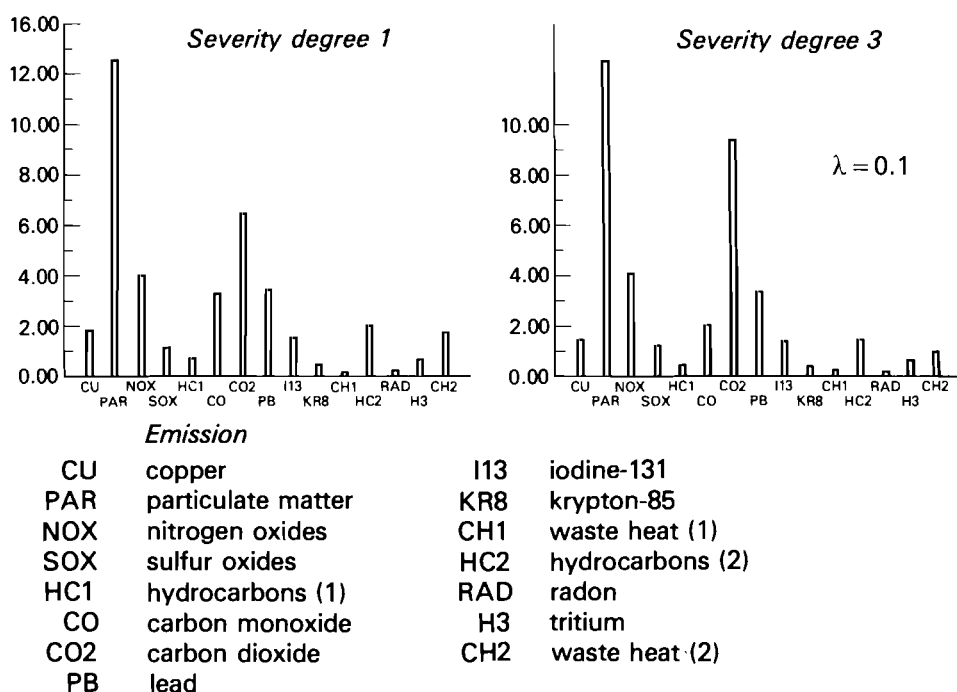
FIGURE 14 The total cost and principal emissions for the cost–environment case.
