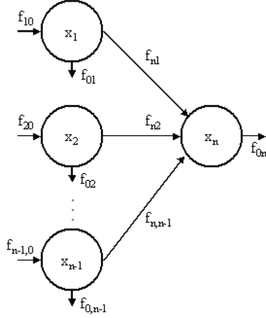
Fig. 9. Parallel interaction in an n -component network with one predator.
