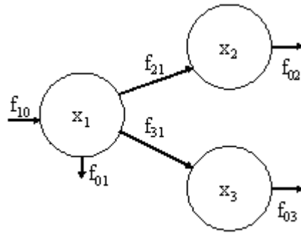
Fig. 2. Competition for a single prey
