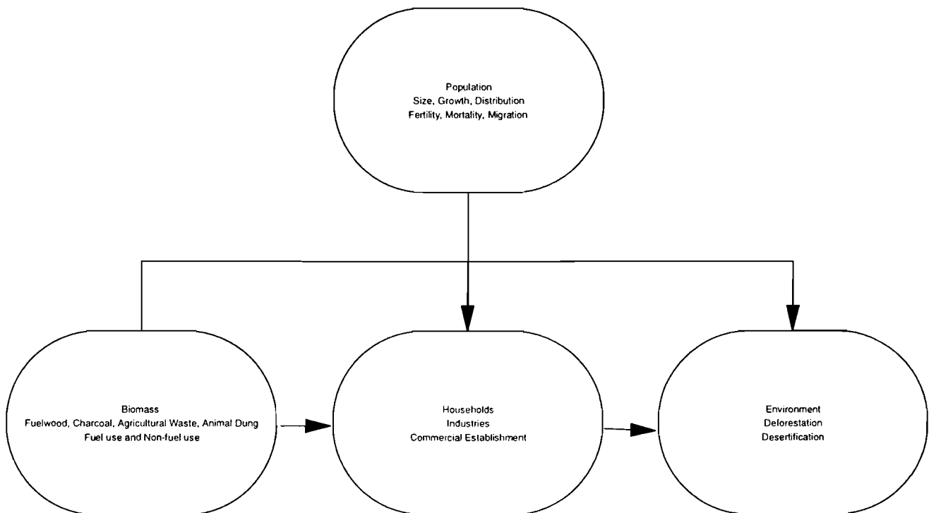
Figure 3. Population-Biomass-Environment Model.
