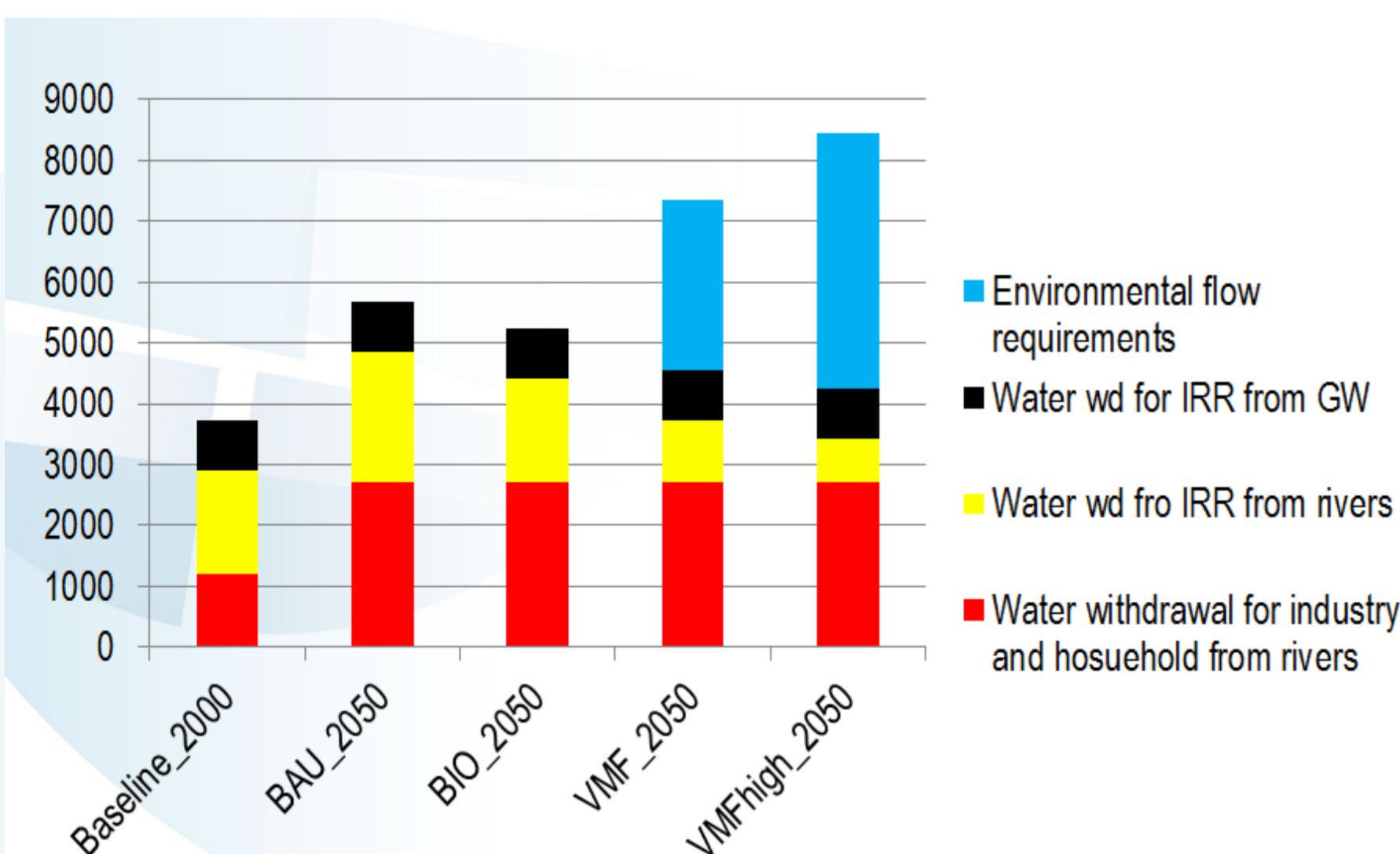
Fig. 4: Global water use prediction with EFR implementation by 2050 (km³ year⁻¹)
