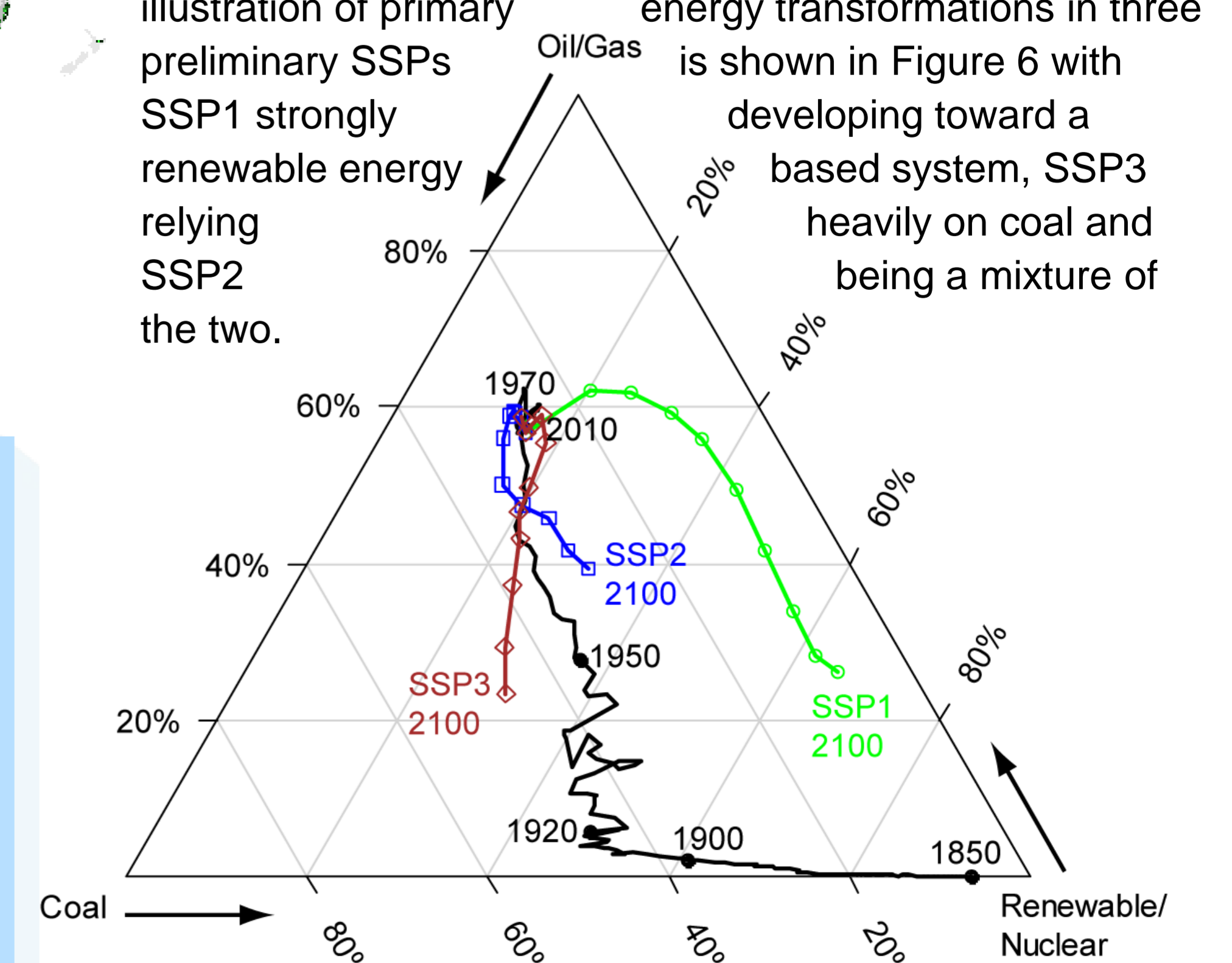
Figure 6: Primary energy transformations across preliminary SSPs developed at IIASA.
