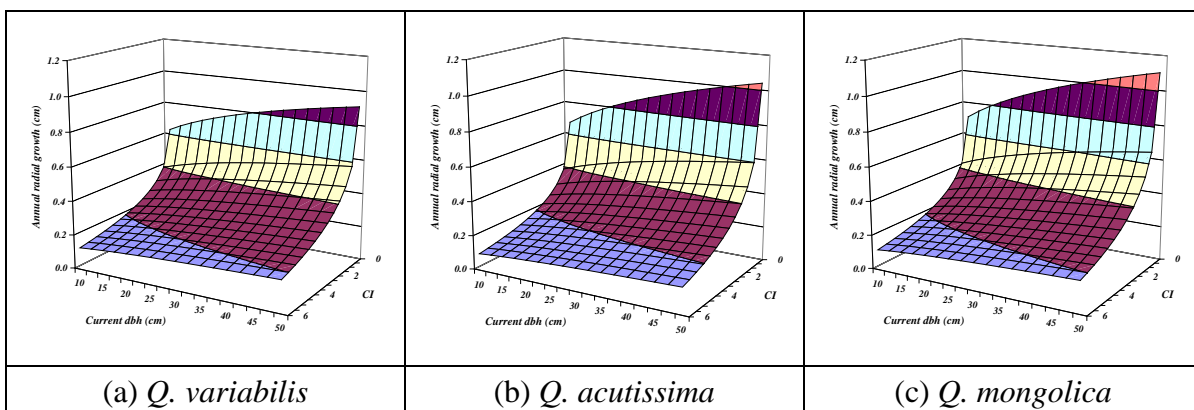
Figure. 4. Annual radial growth for different combinations of Hegyi`s competition index (HgCI) and the current DBH, as simulated using the SQiD model, with a constant tree age of 30 years.
