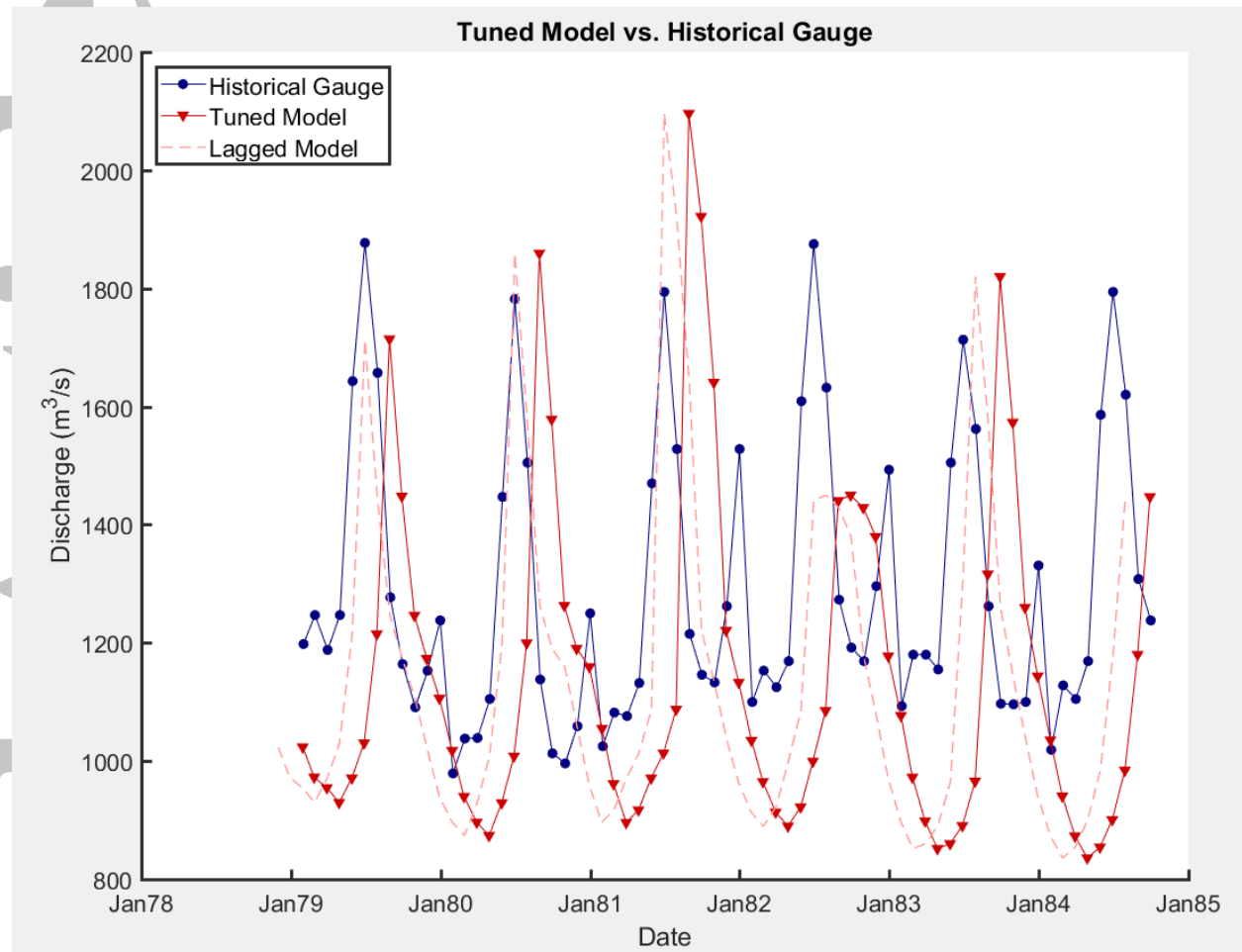
Figure 6. Validation of tuned hydrograph. The monthly comparison shown here indicates that the modelled hydrograph has a one to two-month seasonal time lag for peak flows and has an RMSE of 449 \text{ m}^3/\text{s} and mean and standard deviation of residuals of -145 and 417 \text{ m}^3/\text{s} , respectively. Lagging the model by two months reduces the RMSE to 270 \text{ m}^3/\text{s} . This contrasts sharply with uncalibrated model results that were an order of magnitude larger than gauge flows.
