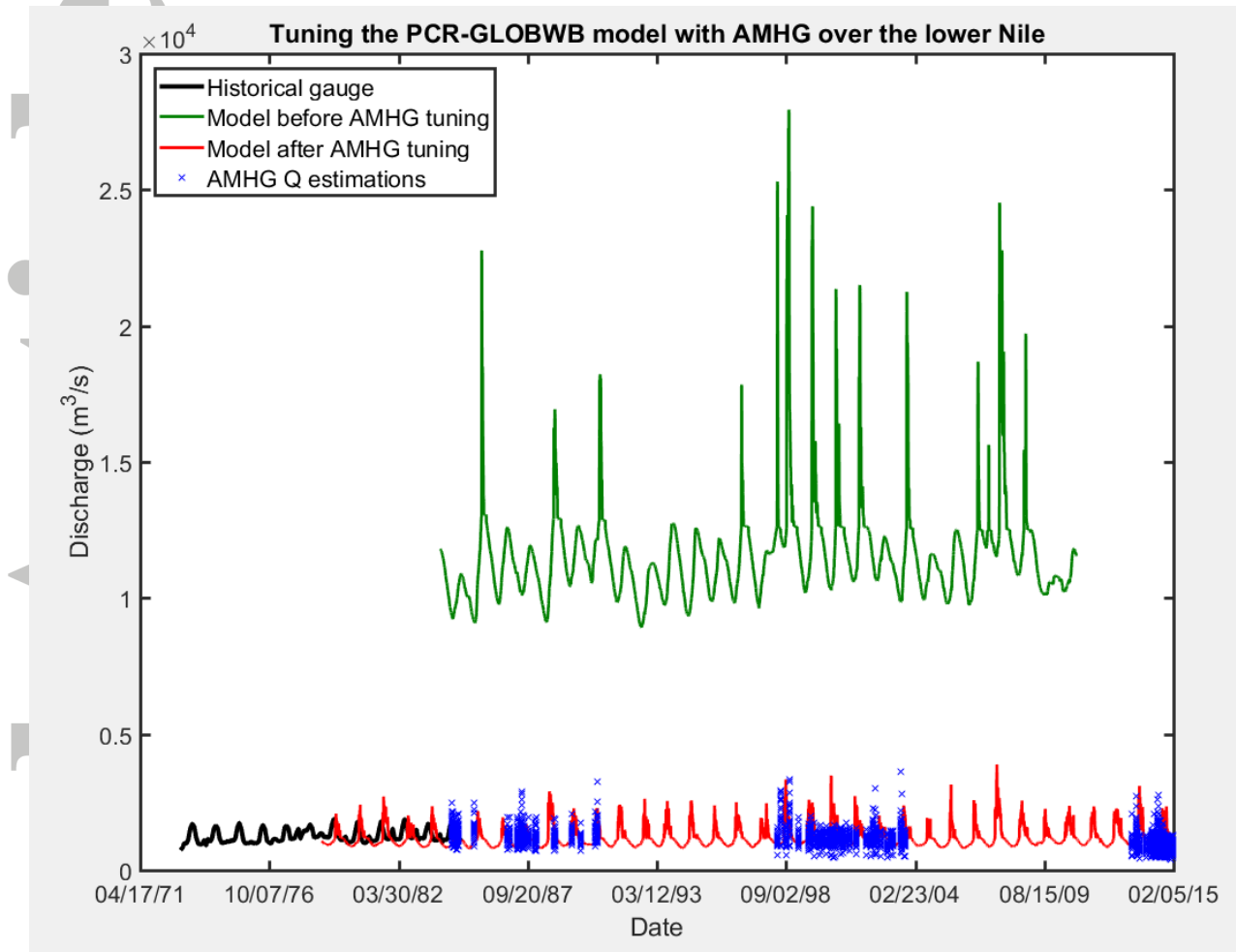
Figure 4. Tuning PCR-GLOBWB with AMHG. This figure shows the substantial improvement gained when using remotely sensed discharge estimates (blue x) to tune a water balance model of the Nile. The uncalibrated model results (green), which have previously been shown to be accurate for most world basins, are an order of magnitude greater than historical flows (black). After model turning from remote sensing, the new (red) hydrograph shows substantial improvement and agreement with historical gauge flows.
