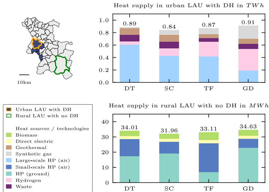
Fig. 2. Comparison of heat supply in an urban LAU with district heating ('Salzburg' city) and in a rural LAU with no district heating ('Abtenau'). Top right: Mix of heat sources in the four different scenarios used in district heating. Bottom right: Mix of heat sources used to supply heat demands decentralized/on-site.
