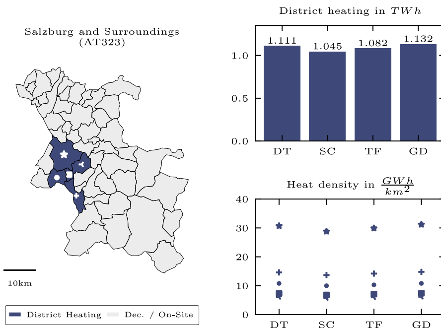
Fig. 1. District heating and decentralized/on-site heat supply in the representative NUTS3 region (incl. LAUs/communities) ‘Salzburg and Surroundings’ (AT323). Left: LAUs with district heating or on-site heat supply. Top right: Total amount of district heating in the four different scenarios. Bottom right: heat density of district heating in the four different scenarios.
