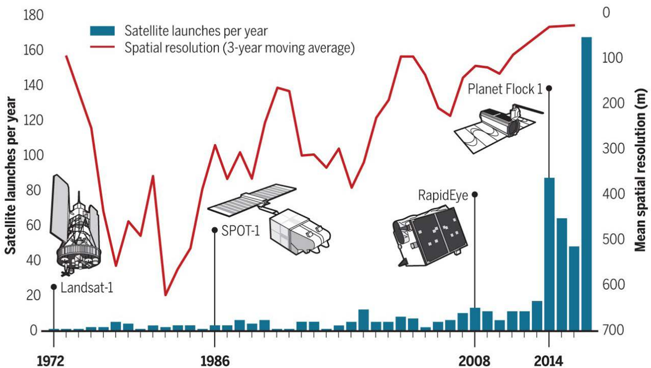
Figure 4: Trends in earth observation satellites. Data reflect 488 earth observation satellites launched since 1972 by commercial and government providers (excluding military). 47
