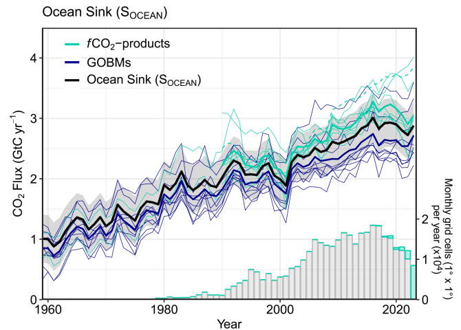
Figure 11. Comparison of the anthropogenic atmosphere–ocean CO 2 flux showing the budget values of S_{\text{OCEAN}} (black; with the uncertainty in grey shading), individual ocean models (royal blue), and the ocean f\text{CO}_2 products (cyan; with UExp-FFN-U, previously Watson et al. (2020), in a dashed line as it is not used for ensemble mean). Two f\text{CO}_2 products (Jena-MLS, LDEO-HPD) extend back to 1959. The f\text{CO}_2 products were adjusted for the pre-industrial ocean source of CO 2 from river input to the ocean by subtracting a source of 0.65 \text{ GtC yr}^{-1} to make them comparable to S_{\text{OCEAN}} (see Sect. 2.5). The bar plot in the lower right illustrates the number of monthly gridded values in the SOCAT v2024 database (Bakker et al., 2024). Grey bars indicate the number of grid cells in SOCAT v2023, and coloured bars indicate the newly added grid cells in v2024.
