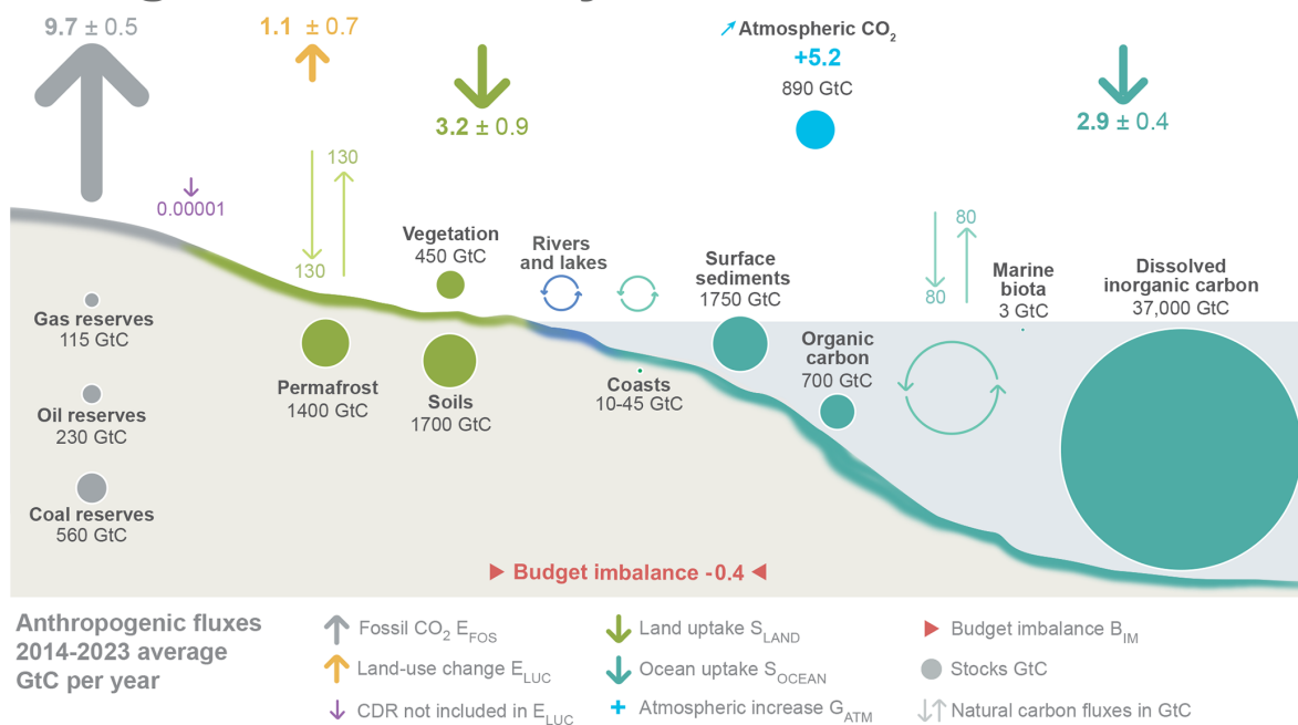
Figure 2. Schematic representation of the overall perturbation of the global carbon cycle caused by anthropogenic activities, averaged globally for the decade 2014–2023. See legend for the corresponding arrows. Flux estimates and their 1 standard deviation uncertainty are as reported in Table 7. The CDR estimate is for the year 2023 only. The uncertainty in the atmospheric CO 2 growth rate is very small ( \pm 0.02 \text{ GtC yr}^{-1} ) and is neglected for the figure. The anthropogenic perturbation occurs on top of an active carbon cycle, with fluxes and stocks represented in the background and taken from Canadell et al. (2021) for all numbers, except for the carbon stocks in coasts, which is from a literature review of coastal marine sediments (Price and Warren, 2016). Fluxes are in gigatonnes of carbon per year ( \text{GtC yr}^{-1} ) and reservoirs in gigatonnes of carbon (GtC). This figure was produced by Nigel Hawtin.
