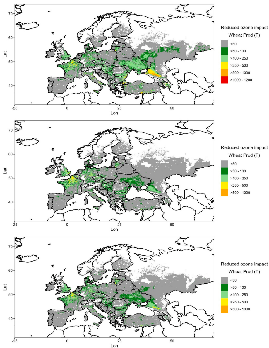
Fig. 4. Additional avoided wheat production losses due to ozone uptake per 0.1° grid cell using the LOW emissions scenario compared to that for current legislation for a) non-methane emissions within the region and b) non-methane emissions from the rest of the world only and c) global methane emissions in 2050. Map lines delineate study areas and do not necessarily depict accepted national boundaries.
