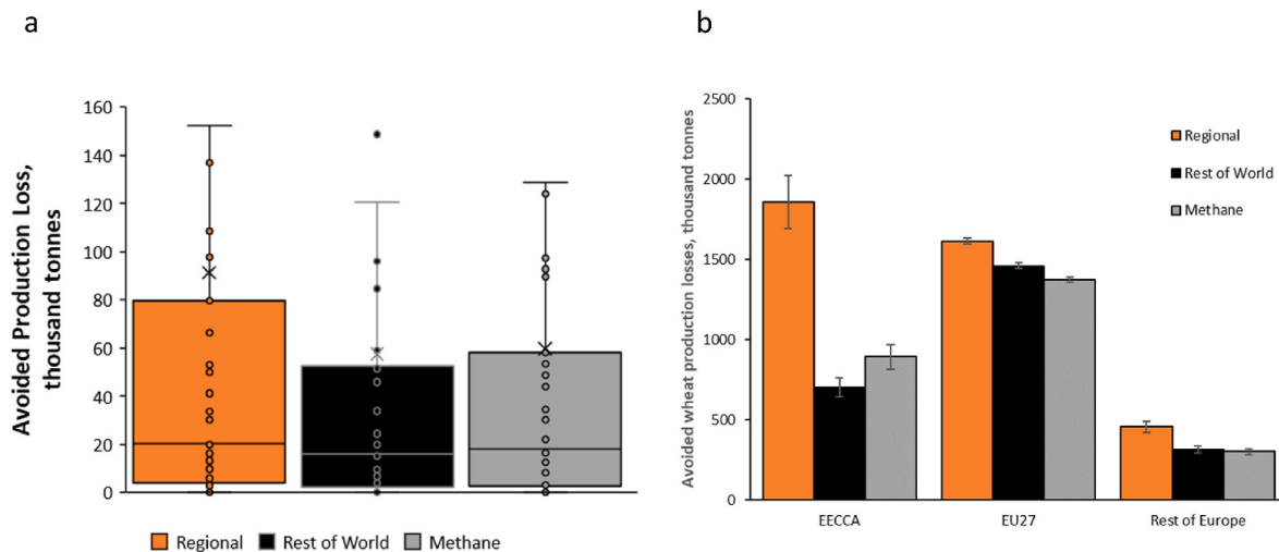
Fig. 6. A) Box plot of avoided wheat production losses per country in the domain from reductions in non-methane emissions within the region, reductions in non-methane emissions in the rest of the world (only) and global reductions in methane emissions (using the LOW scenario), compared to current legislation in 2050. Note the y-axis scale has been constrained for clarity, with the highest outlier points not shown. Differences were not statistically significant. B) Sum of avoided wheat losses for EECCA, EU27 countries and the rest of Europe, bars are standard errors. Differences were not significantly different except for within-region non-methane emissions vs global reductions in methane emissions for the EU27 countries ( p = 0.0418 ).
