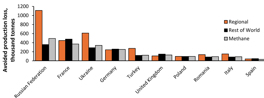
Fig. 5. Additional avoided wheat production losses for the top ten wheat producing countries in the region based on reductions in regional non-methane emissions, rest of the world (only) non-methane emissions, and emissions of methane (using the LOW emissions scenario) compared to the losses from current legislation in the year 2050.
