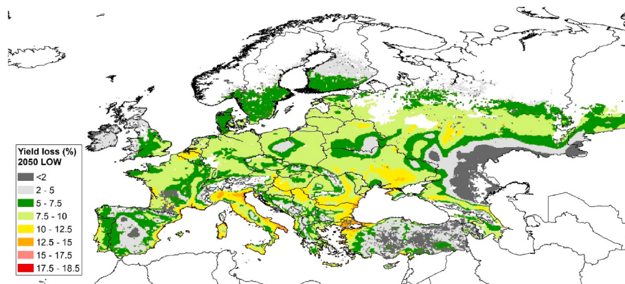
Fig. 7. Percentage yield losses of wheat per grid cell in the LOW scenario compared to those projected based on ozone concentrations in pre-industrial conditions.
