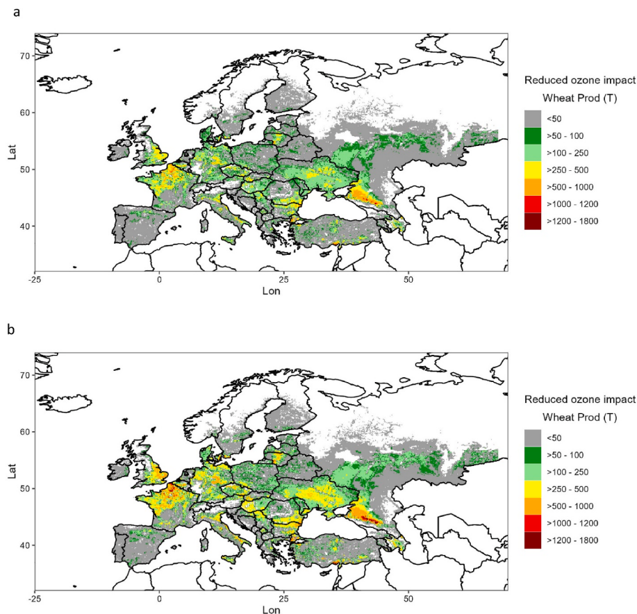
Fig. 1. Additional avoided wheat production losses due to ozone uptake per 0.1° grid cell using the LOW emissions scenario compared to that for current legislation in 2050 for a) non-methane emissions and b) methane and non-methane emissions. Map lines delineate study areas and do not necessarily depict accepted national boundaries.
