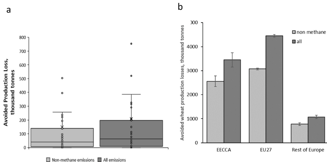
Fig. 3. A) Box-plot of avoided wheat production losses per country in the domain from global non-methane emissions compared with global reductions in all emissions using the LOW scenario, compared to current legislation in 2050. Paired Student t-test p = 0.0007 . Note the y-axis scale has been constrained for clarity, with the highest outlier points not shown. B) Total avoided wheat production loss for EECCA vs EU27 vs rest of Europe, bars are standard errors. Differences are statistically significant for EU27 only ( t = -3.2181 , p = 0.0034 ).
