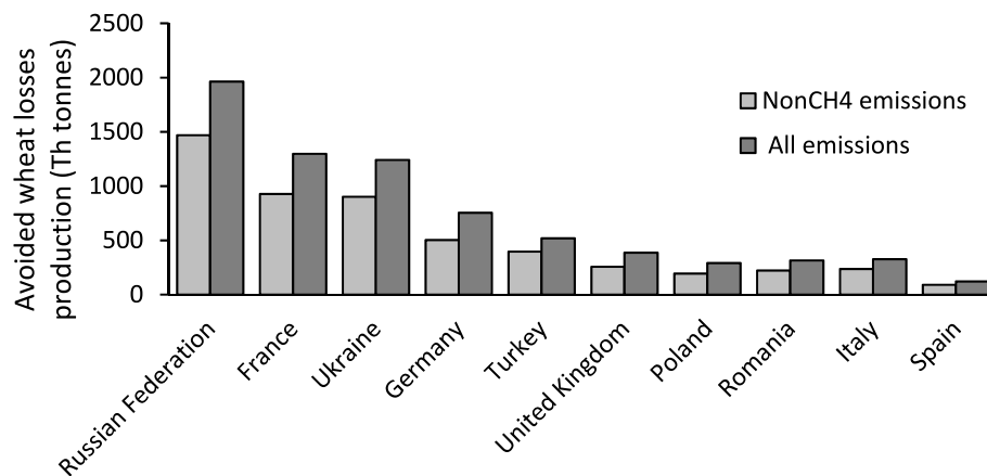
Fig. 2. Additional avoided wheat production losses for year 2050 for the top ten wheat producing countries in the region based on reductions in global non-methane emissions (NonCH4 emissions) and global methane and non-methane emissions (All emissions) – both under the LOW scenario, compared to the losses from the scenario using current legislation.
