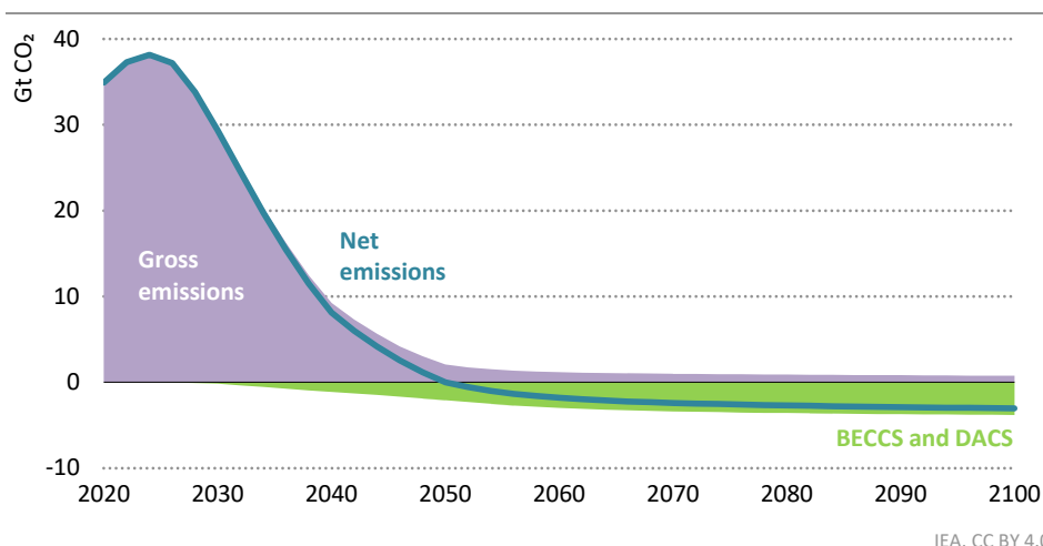
Figure 7.8 ▶ Global gross and net energy-related CO 2 emissions in the NZE Scenario, 2020-2100
