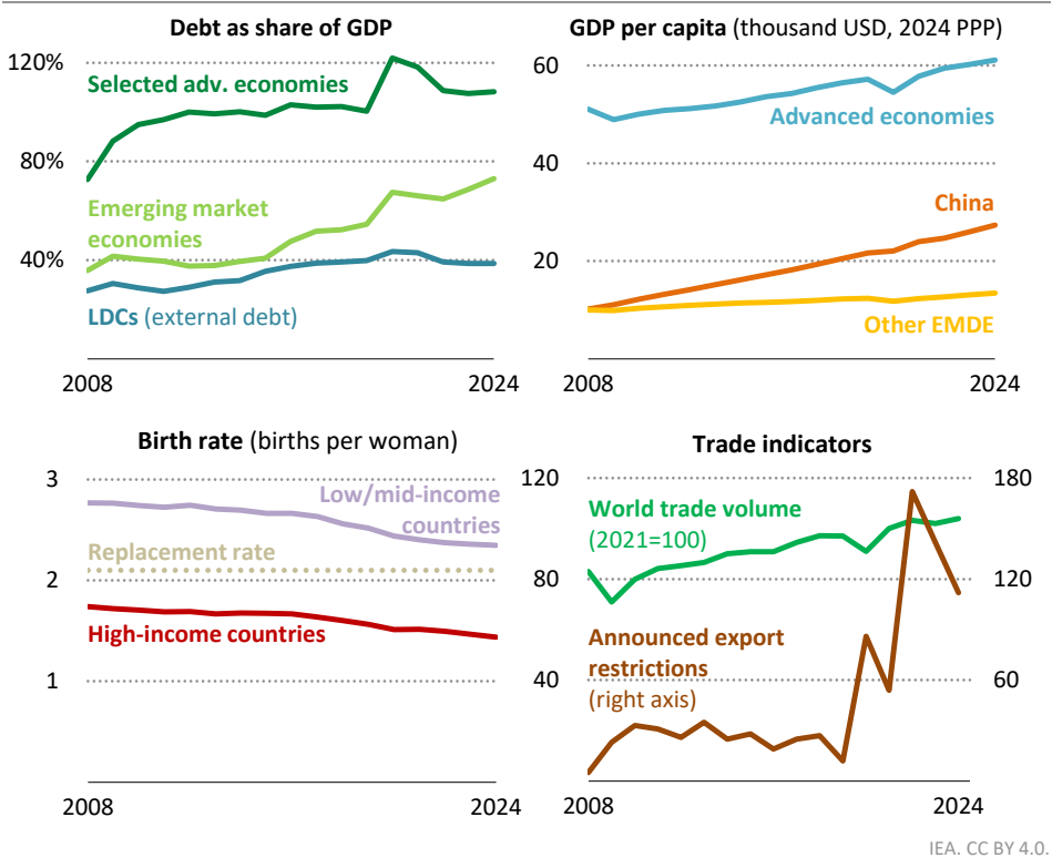
Figure 2.8 ▶ Key trends influencing the global economy, 2008-2024
