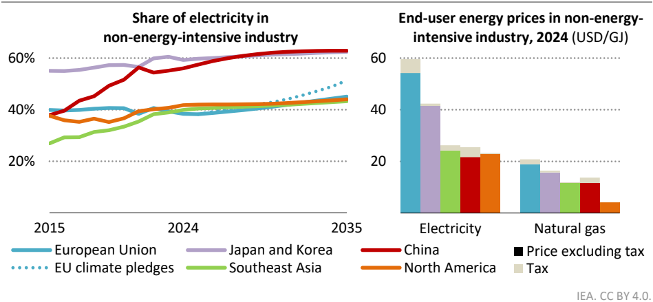
Figure 8.14 ▶ Electrification and end-user prices in non-energy-intensive industry in selected regions in the STEPS, 2015-2035
