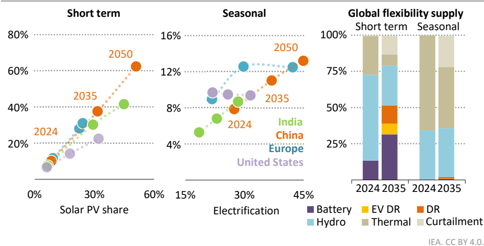
Figure 5.12 ▶ Short-term and seasonal flexibility needs in selected countries, 2024-2050, and global flexibility supply in the STEPS, 2024 and 2035
