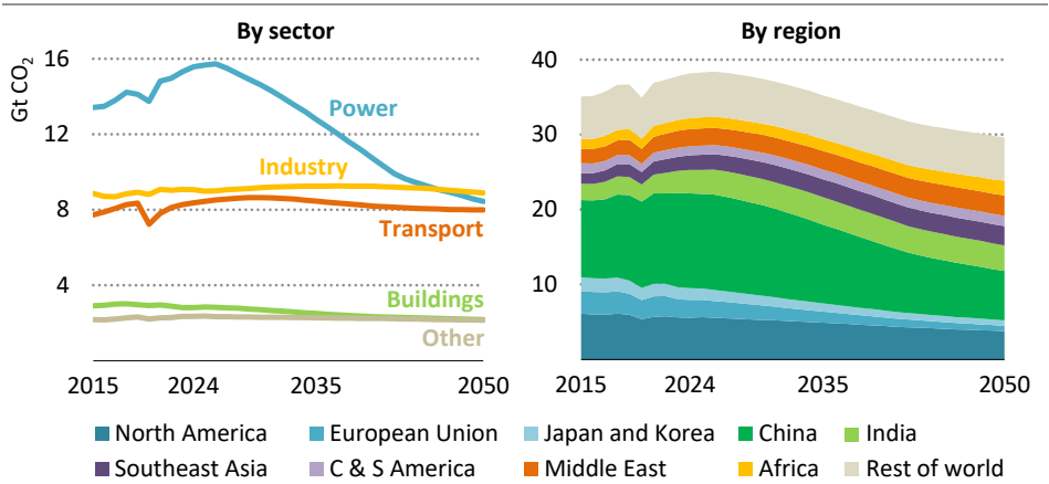
Figure 4.3 ▶ CO 2 emissions by sector and region in the STEPS, 2015-2050
