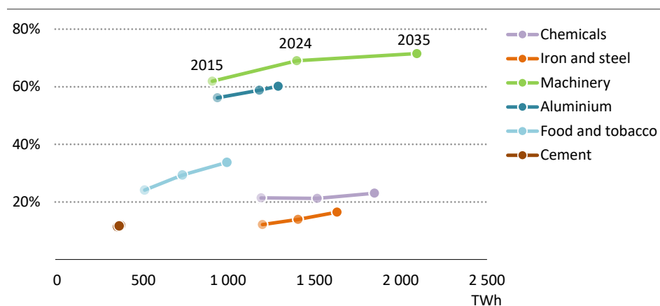
Figure 4.17 ▶ Electricity demand and share of electrification for selected industrial sub-sectors in the STEPS, 2015-2035
