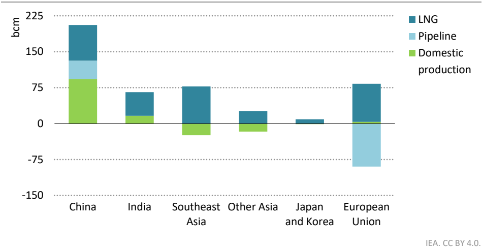
Figure 3.39 ▶ Change in natural gas supply balance in selected regions in the CPS, 2024-2035
