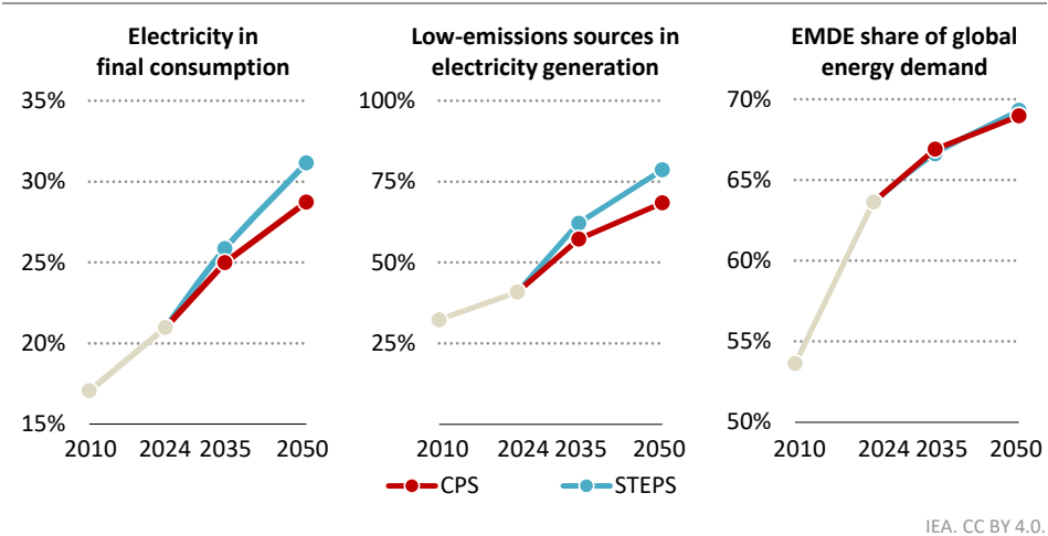
Figure 5.4 ▶ Selected energy indicators by scenario to 2050
