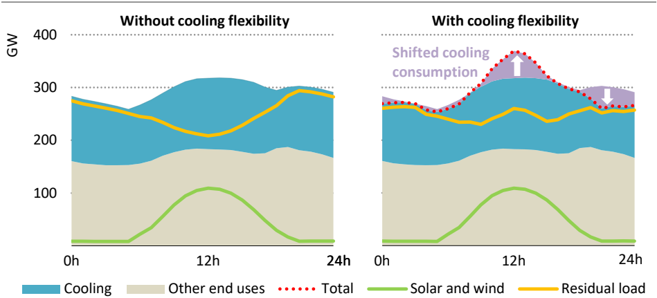
Figure 8.22 ▶ Average summer daily electricity consumption with and without space cooling flexibility in the Middle East in the STEPS, 2035
