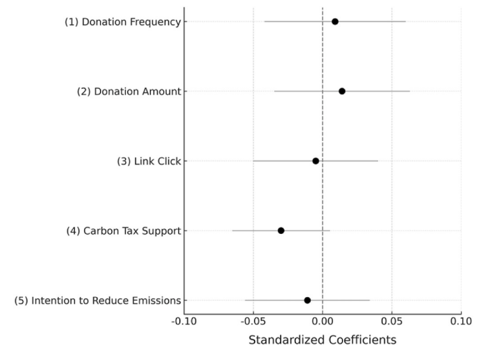
Fig. 3. Forest plot. Notes: Standardised coefficients of treatment effect and standard errors for all five outcome variables.
