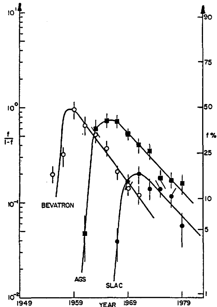
Fig. 7. Just as icecream peddlers, large particle accelerators compete for customers. They can be considered mutants. They come and go in the same way. From: T. W. L. Sanford.
