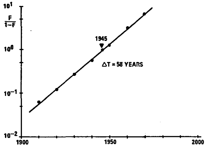
Fig. 3. Just as the iphae of a fungus invade a piece of bread, paved roads spread over the surface of a country. The particular abscissae are for the United States. The equation is always the same.
