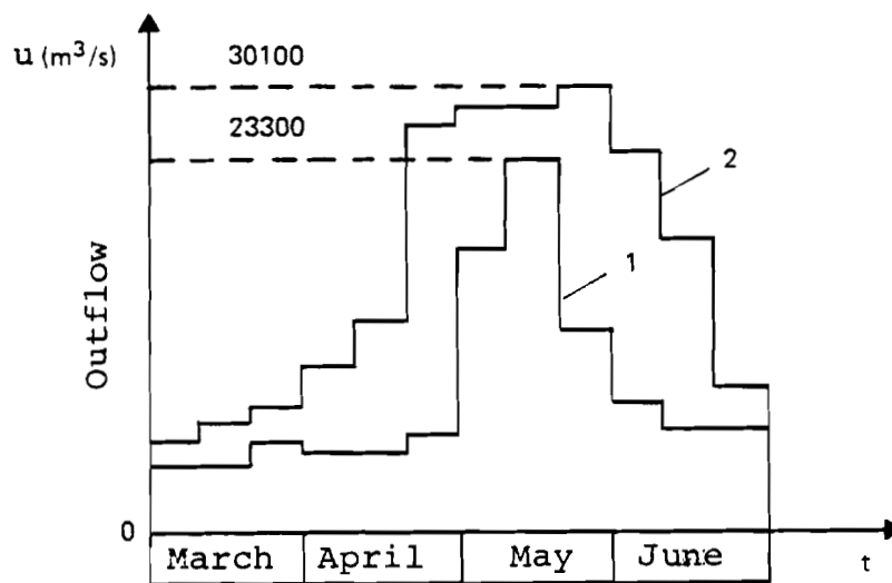
Figure 7. Hydrographies of spring floods for two contrasting years.
