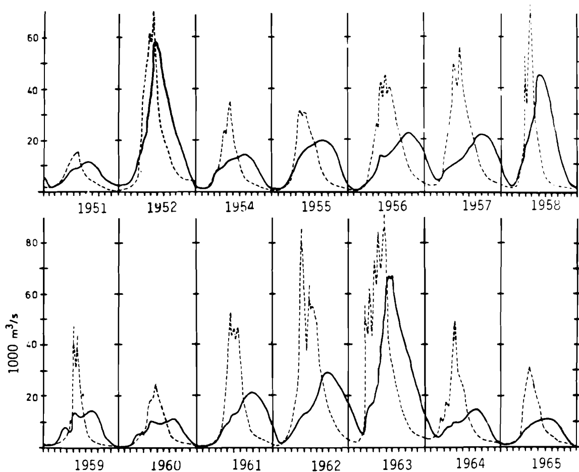
Figure 48. Discharge at Itezihitezhi (broken line) and Kasaka (solid line) from 1950 to 1965 (1952-53 missing). Each hydrological year begins in October (Handlos, 1982).
