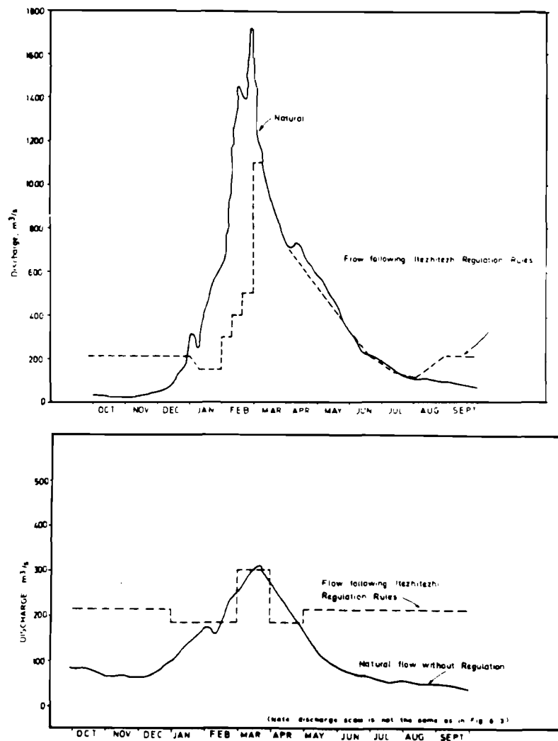
Figure 49. The Kafue hydrograph for an average year at Itzehitezhi (above) and during a dry year (below) (Balasubrahmanyam and Abou-Zeid, 1982b).
