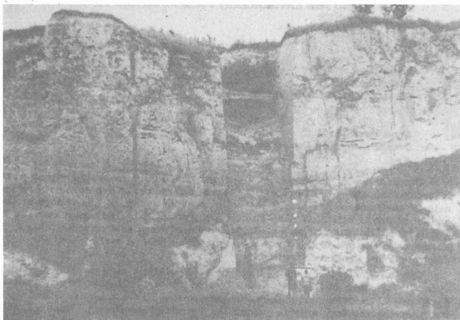
Figure 1. Dolni Vestonice (district of Breclav), Southern Moravia, CSSR. Brickyard exposure at the foot of Palava Mts.: The stratigraphic situation is characterized by alternating yellow loess layers and dark coloured soils.
