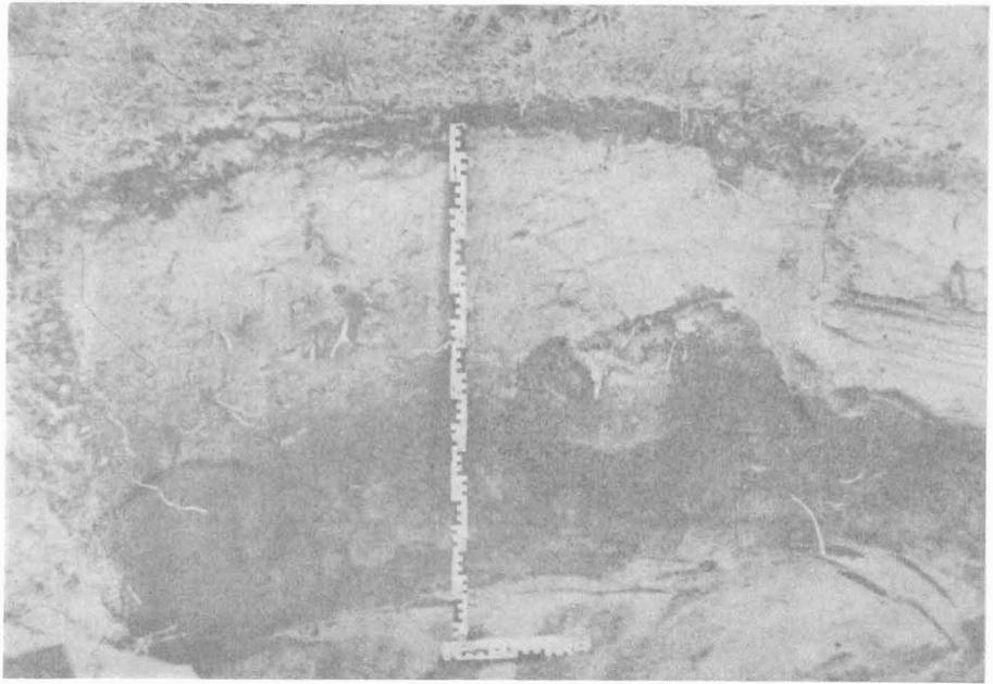
Figure 5 Fischbeck (district of Havelberg), GDR. Dune stratigraphy including the humus horizon (bah) of a buried ranker profile in a sequence of Holocene wind-blown sands. The humus horizon is dated by prehistoric pottery to the so-called Early Iron Age (Pre-Roman period).
