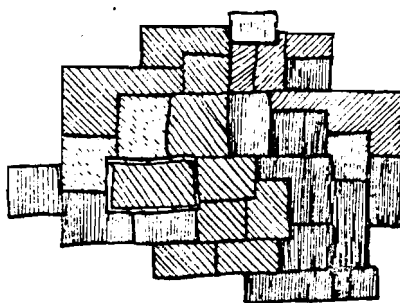
FIGURE 2. Results of cluster analysis for the run without distance-from-the-mine variables.
