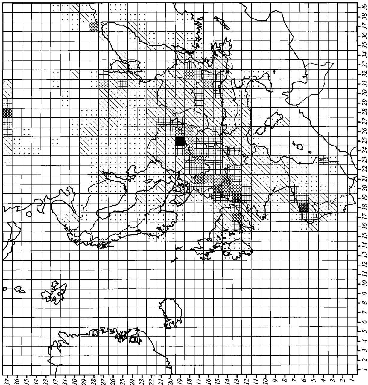
Figure 9. Total deposition of zinc in Europe in 1985 computed by the TRACE model. Units: \text{mg/m}^2 .
