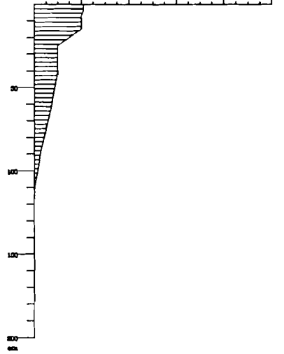
Meadow-chestnut soils
