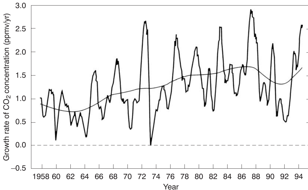
Figure 18: Growth rate of CO 2 concentrations since 1958 in ppmv/yr -1 at the Mouna Loa, Hawaii station. Of importance in the context here are the high growth rates of the late 1980s, the low growth rates of the early 1990s, and the following upturn in the growth rate. The smoothed curve shows the same data but filtered to suppress variations on time scales less than approximately 10 years. Source: Schimel et al. (1996: Figure 2.2).
