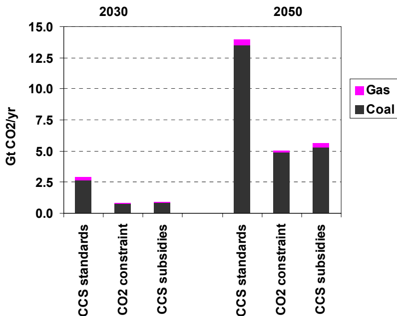
Figure 3.5 Global CO 2 capture from power production by fuel
