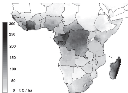
Fig. 5. Above ground Carbon Map – Central Africa (tC/ha in forests).
