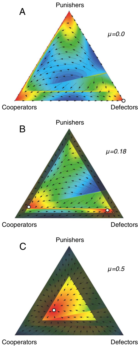
Fig. 1. Dynamics of the system with cooperators, defectors and punishers in the simplex S_3 for different mutation rates. The arrows show the drift term \mathcal{A}_k(\mathbf{x}) of the Fokker–Planck equation, white circles are stable fixed points in the limit M \rightarrow \infty . The discontinuities are a consequence of the strong selection. Blue corresponds to fast dynamics and red to slow dynamics close to the fixed points of the system. The system does typically not access the gray shaded area, because the minimum average fraction of each type because of mutations is \mu/3 . (A) For vanishing mutation probability ( \mu \rightarrow 0 ), there is only 1 stable fixed point in the defector corner. (B) For \mu = 0.2 , there are 2 stable fixed points, one close to the cooperator corner and one close to the defector corner. The population noise can drive the system from the vicinity of one of these points to the other, which makes an analytical description of the dynamics difficult. (C) For \mu = 0.5 , there is only a single stable fixed point, which is closest to the cooperator corner—thus, cooperators prevail for high mutation rates. We use the position of this fixed point as an estimate for the average abundance of the strategies, see Fig. 2 [parameters: M = 100 , N = 5 , r = 3 , c = 1 ; \beta = 1 , \gamma = 0.3 ; \sigma = 1 , graphical output based on the Dynamo software (37)].
