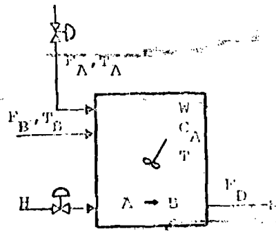
Fig.11 A stirred-tank reactor.
