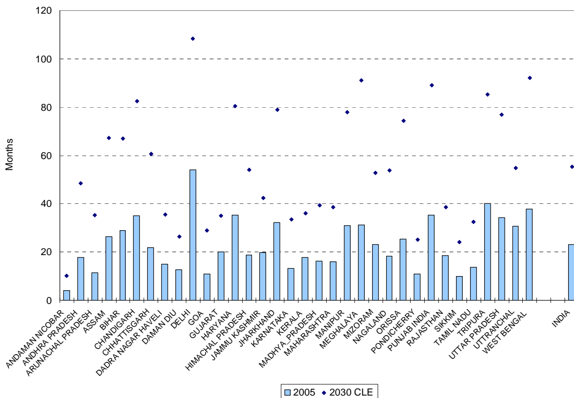
Figure 3.6: Loss in statistical life expectancy attributable to the outdoor exposure of fine particulate matter computed for 2005 and the 2030 baseline projection (central estimate)
