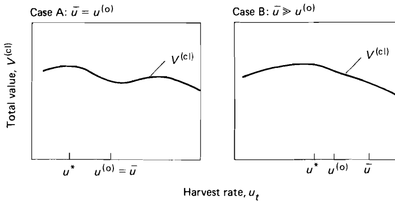
Figure 4.1. Examples of how the long-term value of harvests can be broken down into components as functions of harvest rate. The total value is V^{(cl)} . In case A, higher probing values away from the nominal u^{(o)} imply that the optimum u^* is far below u^{(o)} . In case B, even using u^{(o)} is informative since it is far from the historical average \bar{u} . (Part of Figure 9.10 in Adaptive Management of Renewable Resources .)
