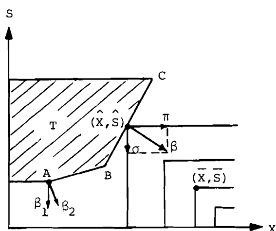
Figure 5. The determination of efficient points.
