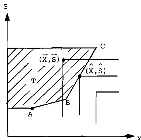
Figure 5. The determination of efficient points.
