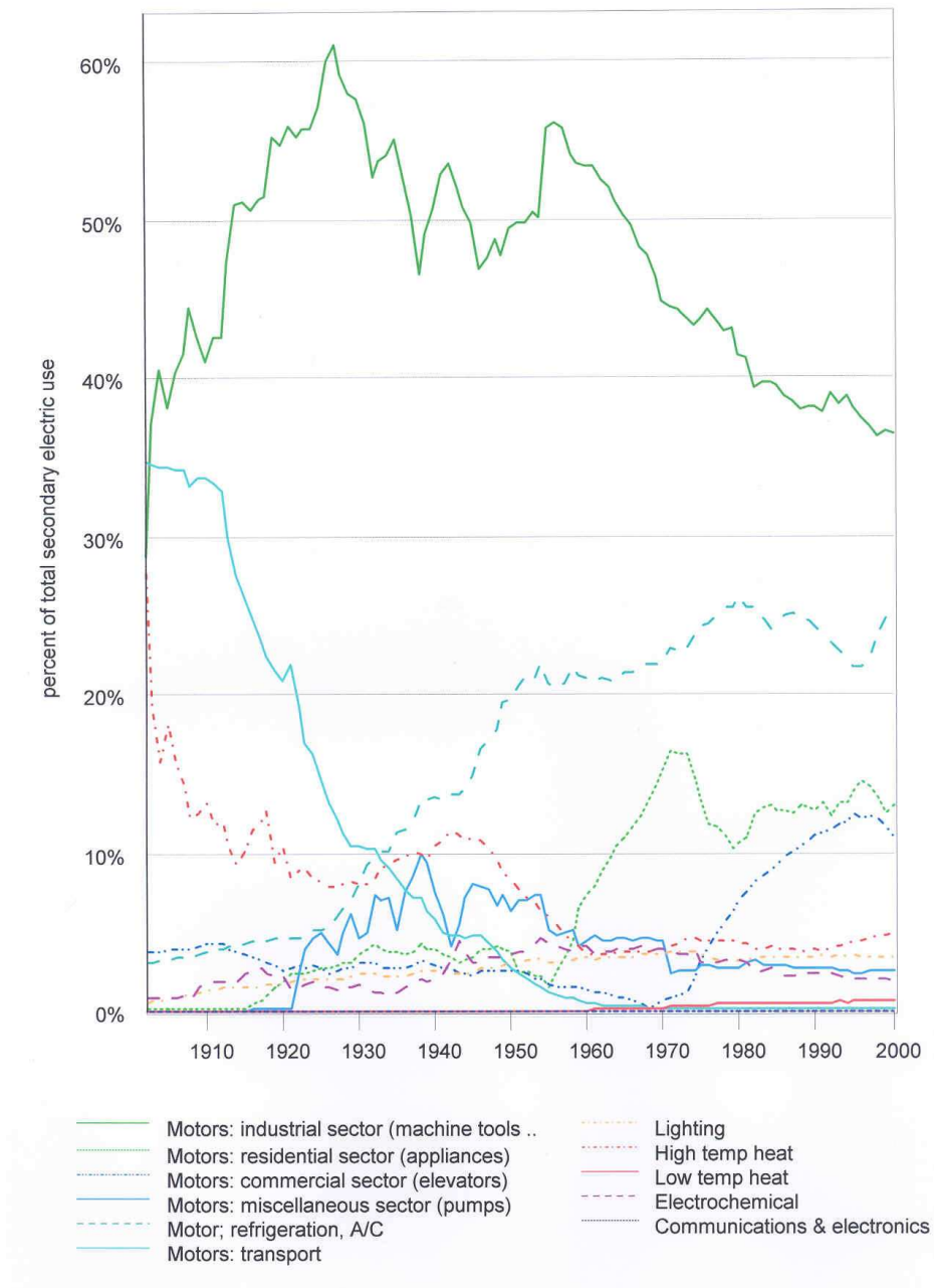
Figure 5: Secondary electrical work by function as percentage of total secondary electrical work, USA 1902-2000.
