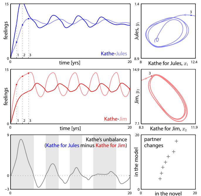
FIG. 5. The love story predicted by the validated model ( \varepsilon and \delta at the white dot in Fig. 4, other parameters as in Table 1). (Top panels) Time series of the feelings and trajectory projections in the planes of the Kathe-Jules and Kathe-Jim submodels. (Bottom panels) Kathe’s preference and comparison with the novel.
