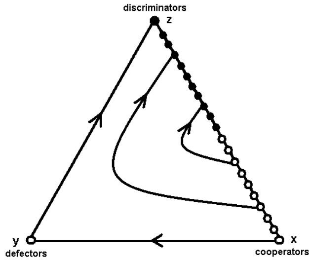
Figure 4: The replicator dynamics of direct reciprocity, in the absence of errors, i.e. \epsilon = 0 , for w = 1 .
