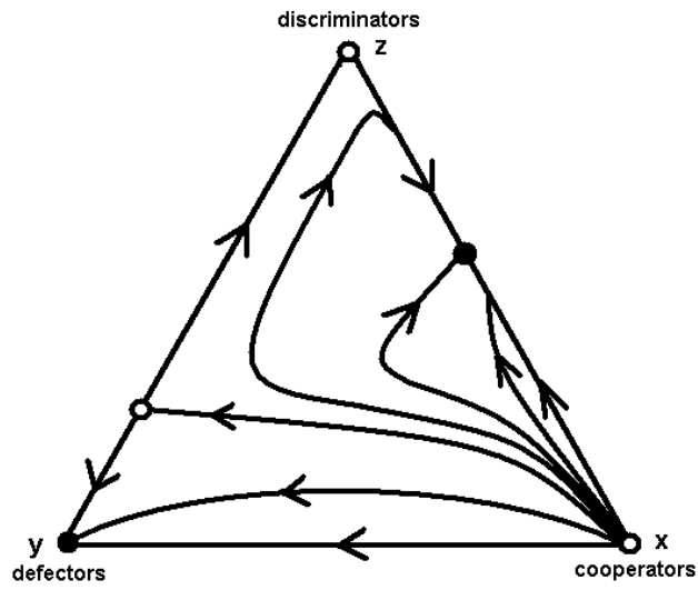
Figure 14: The replicator dynamics of indirect reciprocity if one assumes synchronous rounds, \epsilon > 0 , and a number of rounds which is fixed, or Poisson distributed.
