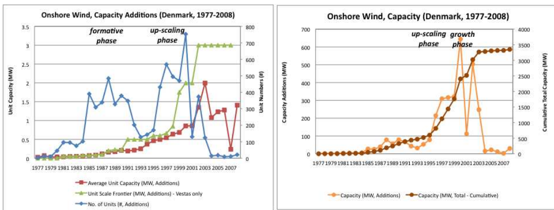
Figure 6. Growth in Onshore Wind Capacity in Denmark Since 1977.
