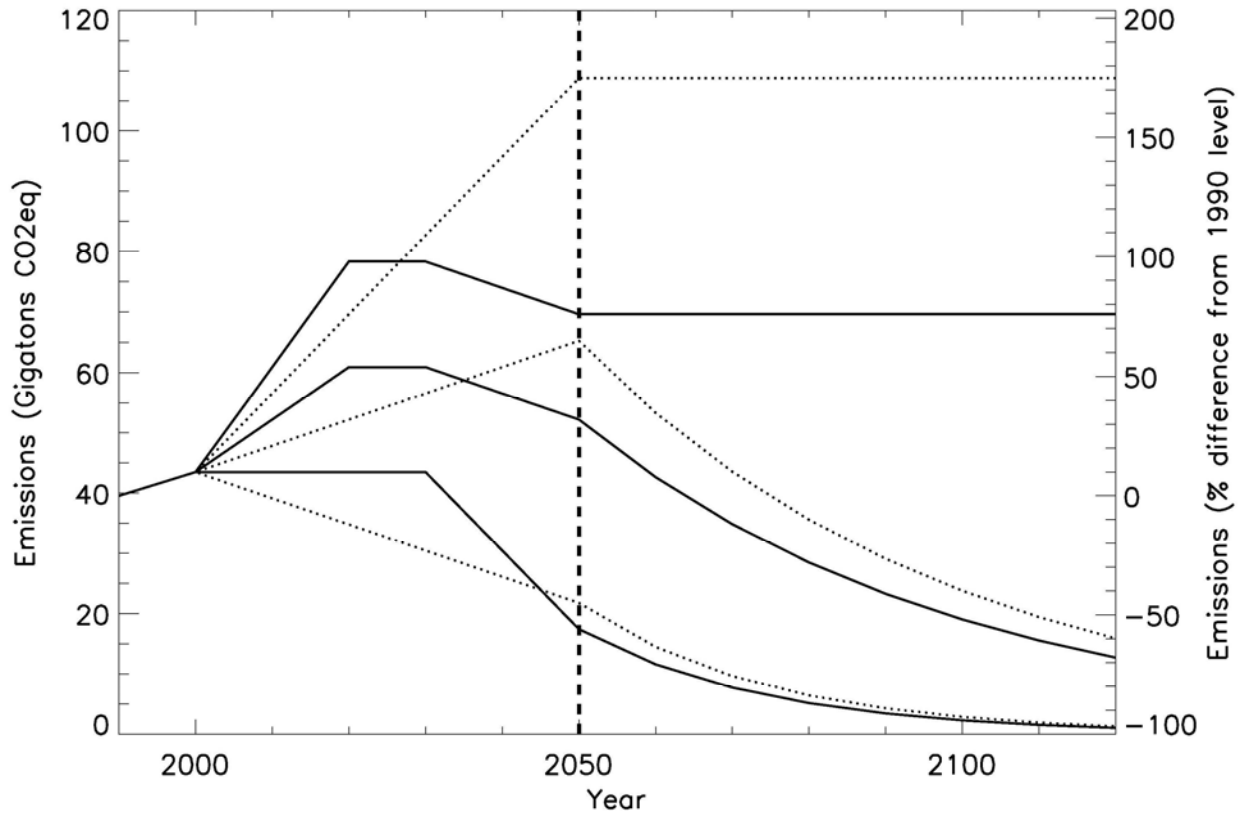
Figure 1. Illustrative global emissions pathways used in the standard analysis (solid curves) and sensitivity analysis (dotted curves). Note that we weight the gases by their global warming potentials (GWPs), with values taken from the IPCC Third Assessment Report (IPCC, 2001), only for the purpose of plotting aggregate emissions in terms of CO 2 equivalents (CO 2 eq); the radiative effect of the gases is calculated explicitly in our climate model and independently of the GWP values. The pathways depicted here bracket the lowest and highest cumulative emissions. Specifically, the three standard curves (from lowest to highest) vary in the following manner: between 2000 and 2020, they increase linearly by 0%, 2%, and 4% of the 2000 level per year; from 2020 to 2030, they are constant; from 2030 to 2050 they decrease linearly by 3%, 1%, and 1% of the 2000 level per year; and after 2050, they decrease exponentially by 4%, 2%, and 0% per year. The three sensitivity curves change linearly by -1%, 1%, and 3% of the 2000 level per year from 2000 to 2050, and then decrease exponentially by 4%, 2%, and 0% per year after 2050.
