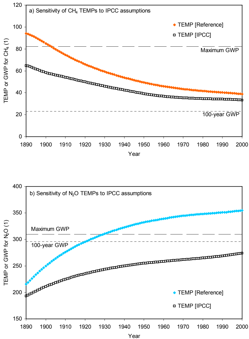
Figures 5a-b. Updating \text{CH}_4 and \text{N}_2\text{O} TEMPs under the assumptions used for IPCC GWP calculations. Backward-looking TEMPs are calculated for every year from 1890 to 2000.
