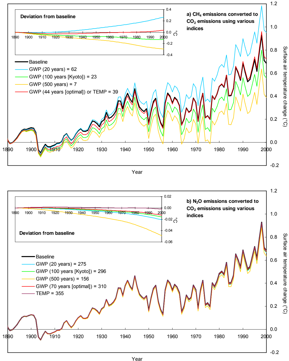
Figures 3a-b. Temperature projections with CH 4 or N 2 O emissions converted using GWPs and TEMPs. The conversions are applied from the year 1890 onward. Baselines are the posterior estimates obtained from the ACC2 inverse calculation. The temperature projection using the CH 4 TEMP is identical with the projection using the optimal-horizon CH 4 GWP.
