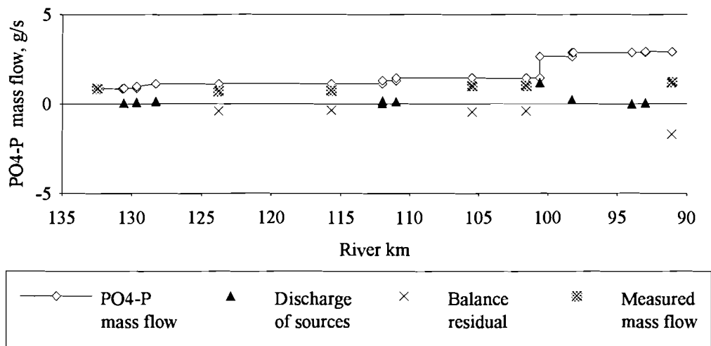
Figure 3.16 Orthophosphate phosphorus mass balance for the upper part of the Nitra River (August 25-26, 1992 experiment)
