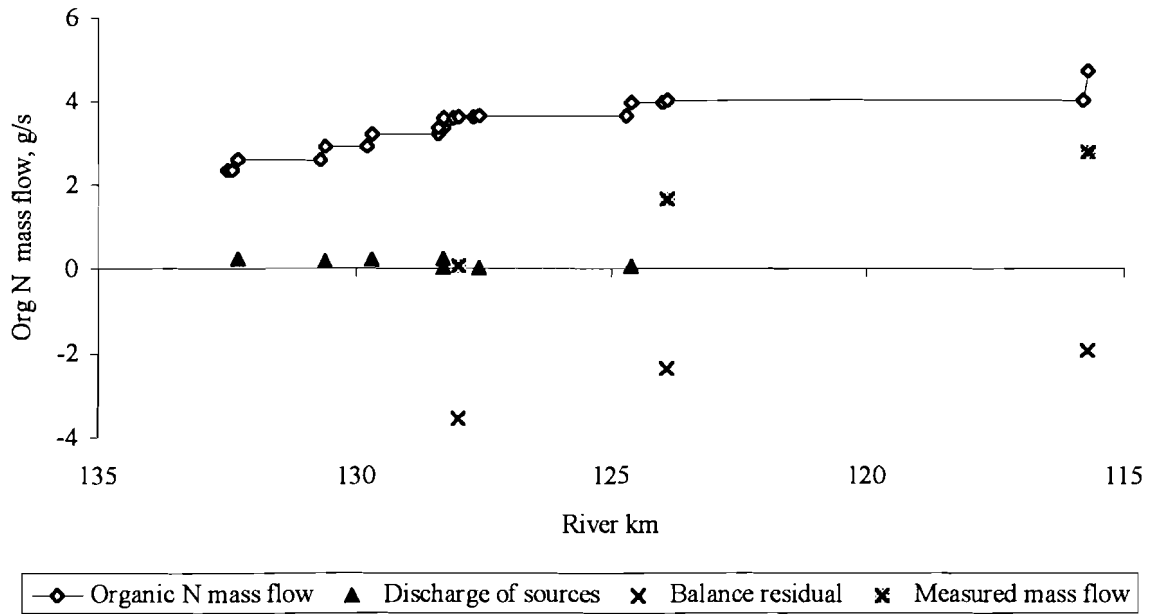
Figure 4.14 Organic nitrogen mass balance for the upper part of the Nitra River (June 1993 experiment)
