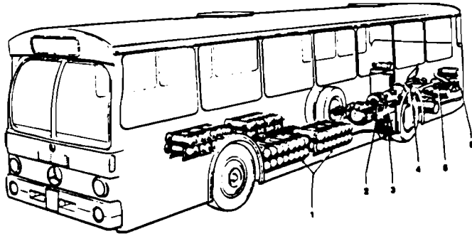
Figure 1. Test Bus Retrofitted to CNG. SOURCE: Christ (1986).
