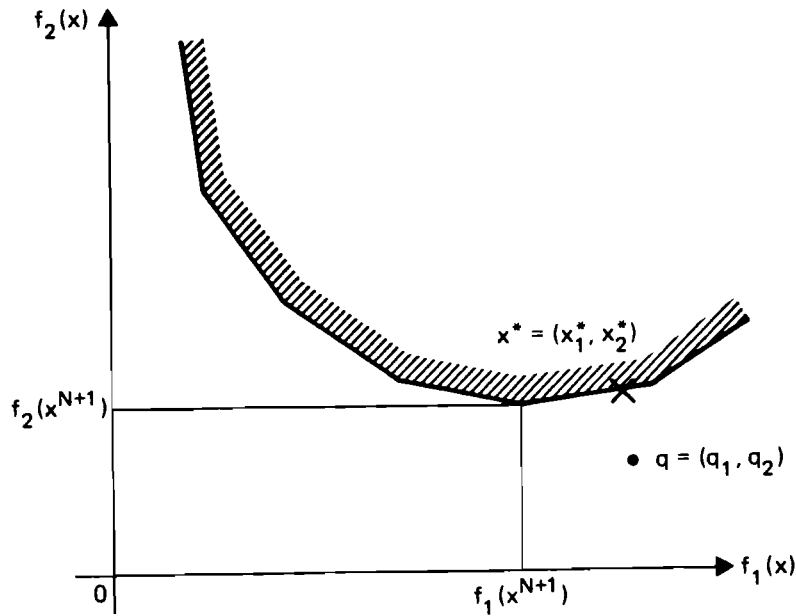
Figure 6. Illustration of the case in which q_1 > f_1(x^{N+1}) holds.
