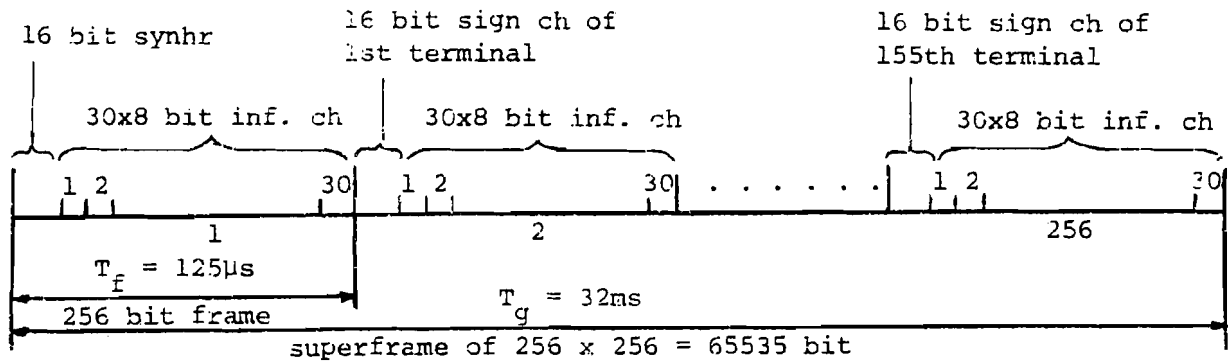
Figure 15. Format of Transmitted Information in IDLS
