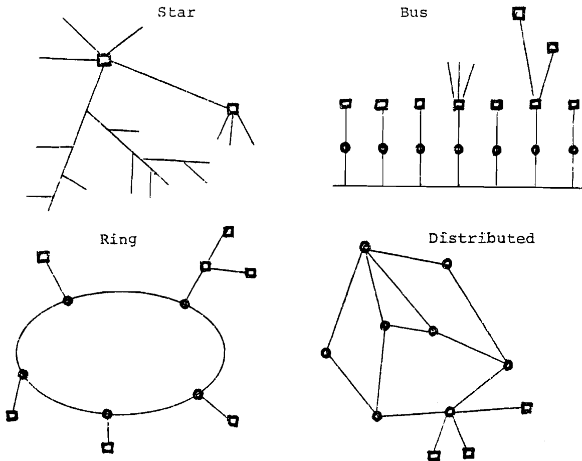
Figure 8. IICN Topology
