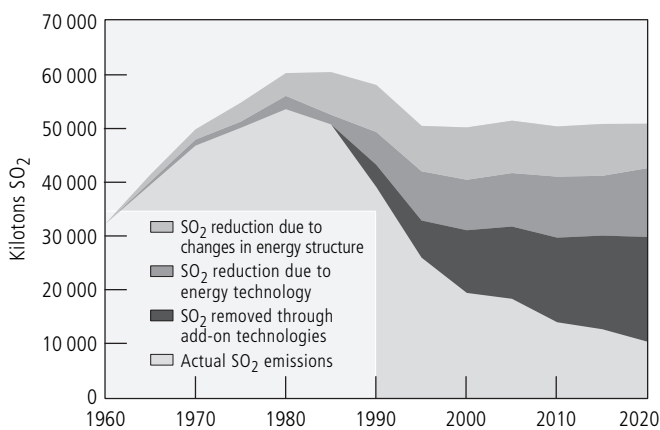
Figure 2. The prevention of sulphur dioxide ( \text{SO}_2 ) emissions in Europe 1960–2020: Actual levels compared to hypothetical levels, taking into account energy consumption growth
