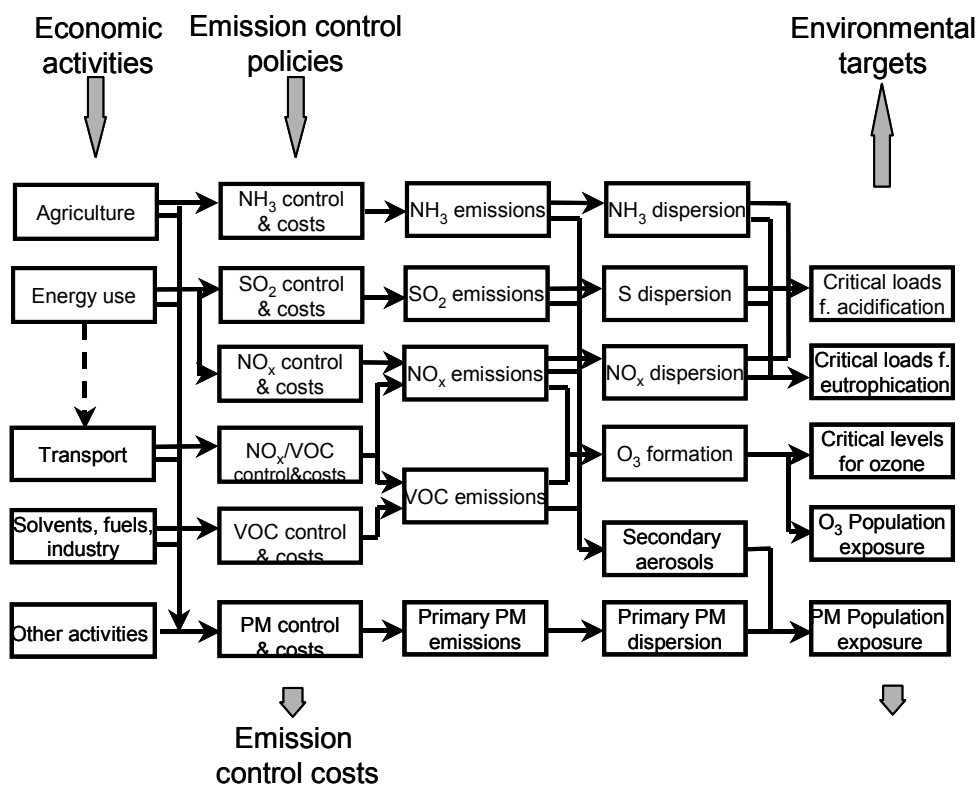
Figure 1. Structure of the RAINS model in 2006
